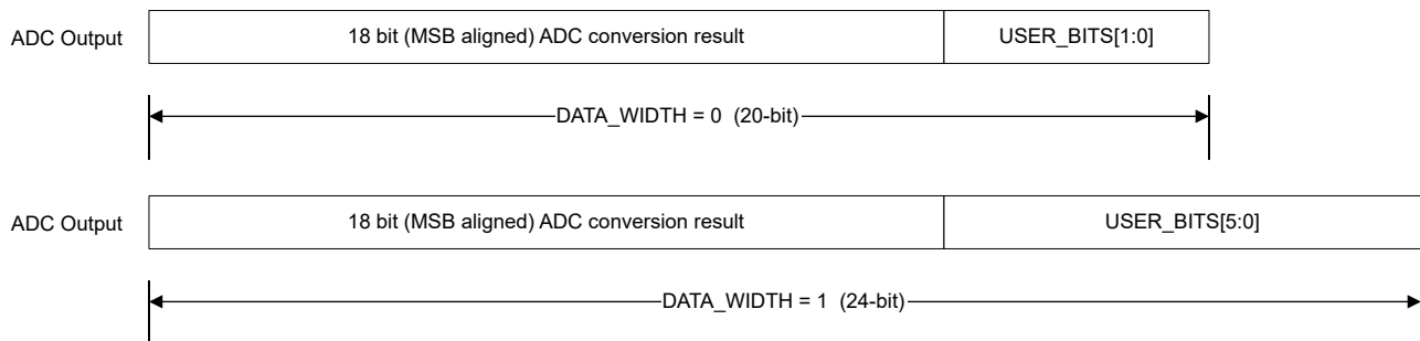
Figure 7-6. Data Frame Width Composition
