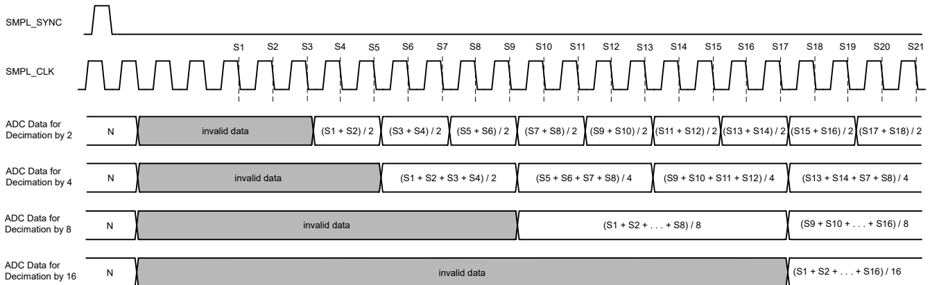
Figure 7-4. Data Output With Decimation
