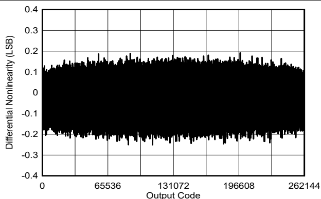
Typical DNL = \pm 0.4\text{LSB}
