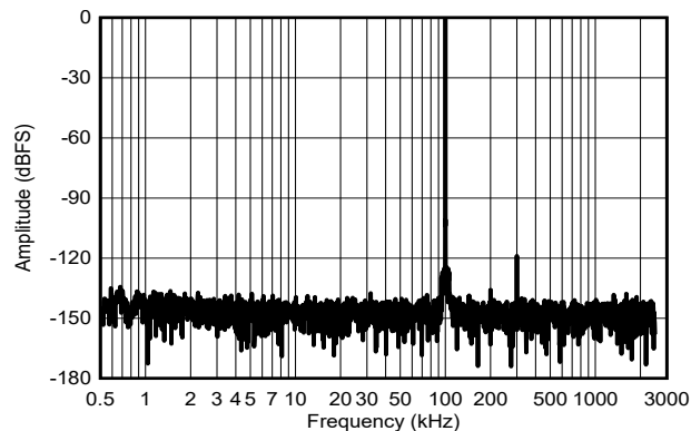
f_{IN} = 100\text{kHz} , SNR = 95.4dBFS, THD = -120dB
