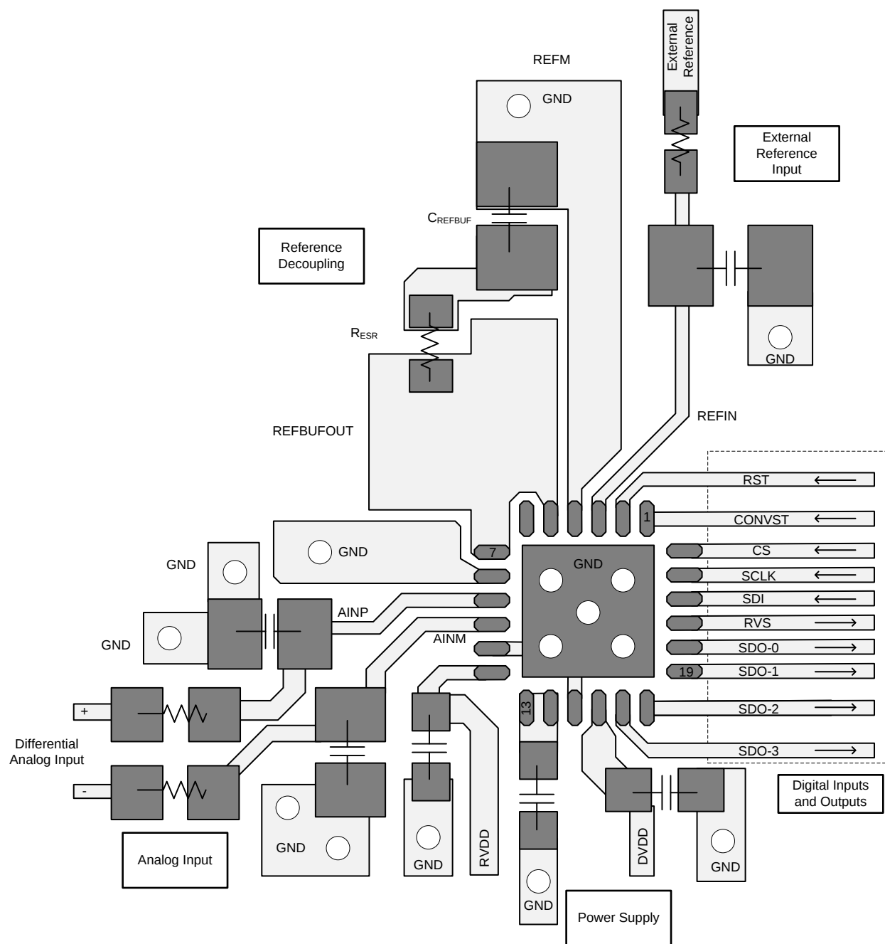
Figure 121. Recommended Layout
