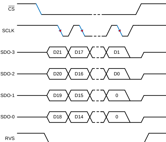
Figure 73. SPI-10-Q-EDL Protocol
