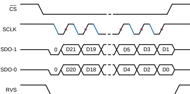
Figure 65. SPI-11-D Protocol
