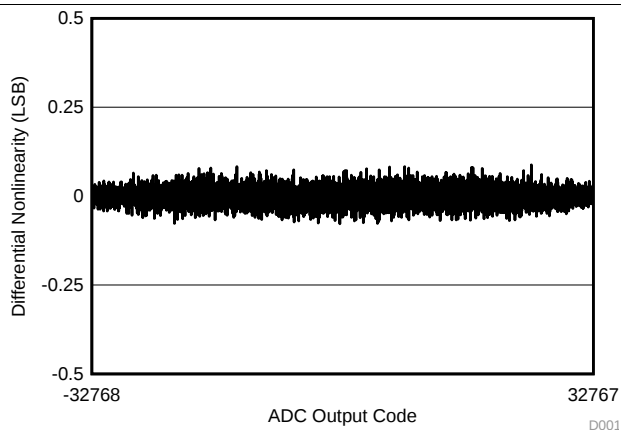
Figure 6. Typical DNL
