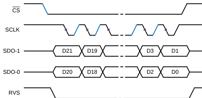
Figure 64. SPI-10-D Protocol
