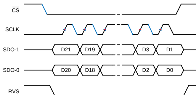
Figure 62. SPI-00-D Protocol
