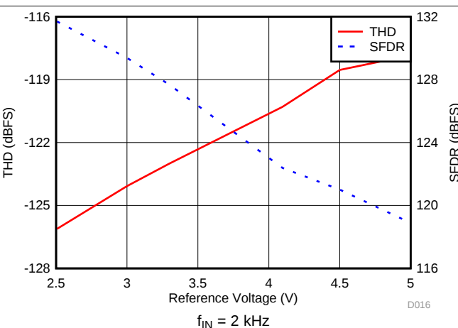
Figure 27. Distortion Performance vs Reference Voltage
