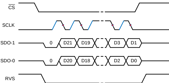
Figure 63. SPI-01-D Protocol
