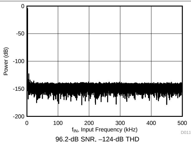
Figure 107. Noise-Performance FFT Plot - ADS8920B
