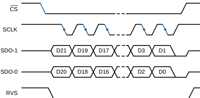
Figure 71. SPI-10-D-EDL Protocol
