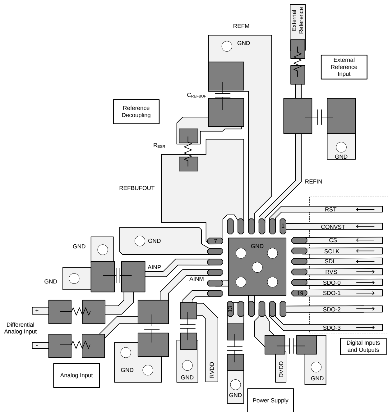
Figure 121. Recommended Layout
