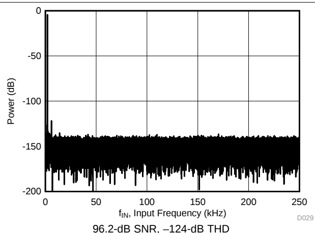
Figure 108. Noise-Performance FFT Plot - ADS8922B
