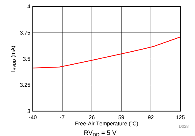
Figure 29. Analog Supply Current vs Temperature
