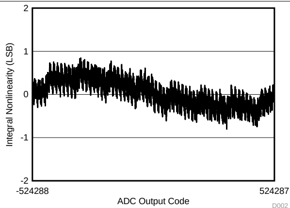
Figure 7. Typical INL
