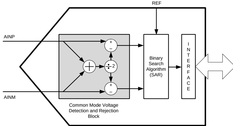
Figure 46. Conceptual Diagram: True Differential Input Structure
