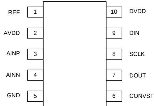
DGS PACKAGE VSSOP-10 (TOP VIEW, Not to Scale)
