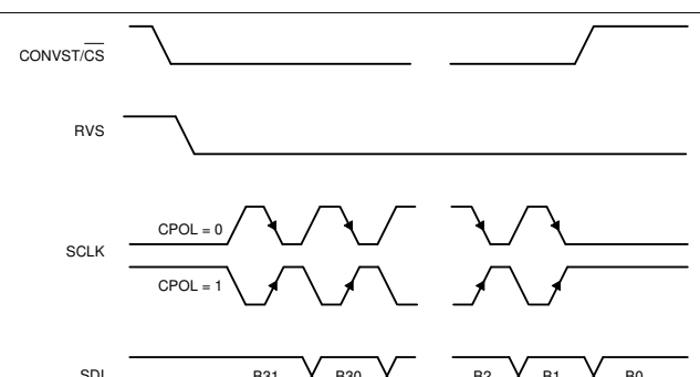
Figure 7-27. Standard SPI Timing Protocol (CPHA = 1, 32 SCLK Cycles)
