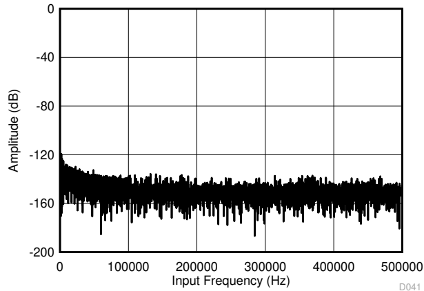
图 6-33. Typical FFT Plot (All Ranges) for the ADS8681
