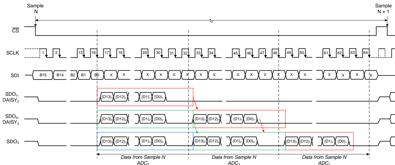
Figure 93. Three Devices Connected in Daisy-Chain Mode Timing Diagram
