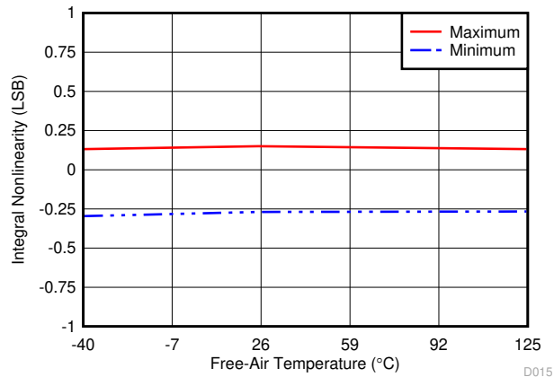
图 6-27. INL vs Temperature (All Unipolar Ranges)
