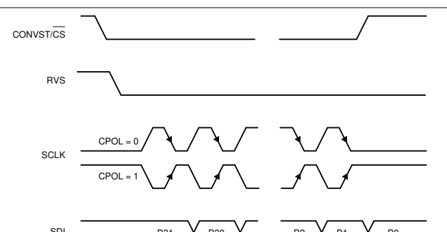
图 7-27. Standard SPI Timing Protocol (CPHA = 1, 32 SCLK Cycles)
