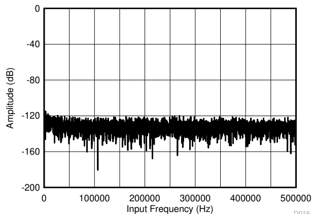
图 6-33. Typical FFT Plot (All Ranges) for the ADS8671
