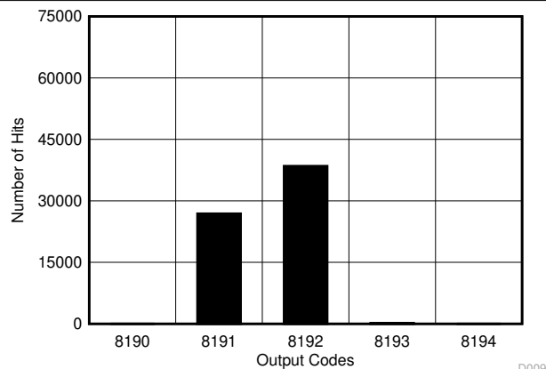
图 6-21. DC Histogram for Mid-Scale Inputs (0 V – 5.12 V)
