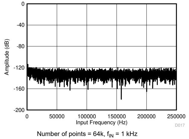
图 6-34. Typical FFT Plot (All Ranges) for the ADS8675
