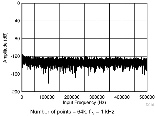
图 6-33. Typical FFT Plot (All Ranges) for the ADS8671
