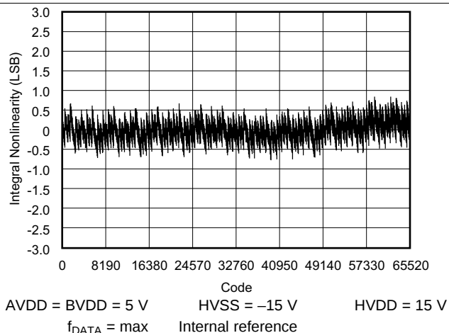
Figure 6. INL vs Code (ADS8556 \pm 5\text{-V}_{IN} Range)
