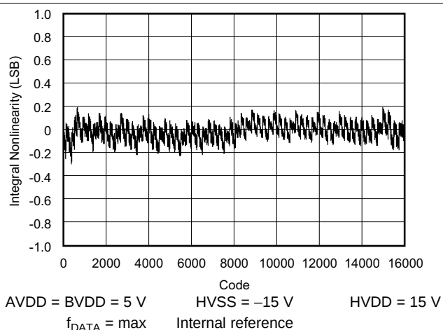
Figure 10. INL vs Code (ADS8557 \pm 5\text{-V}_{IN} Range)
