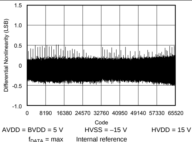
Figure 7. DNL vs Code (ADS8556 \pm 10\text{-V}_{IN} Range)
