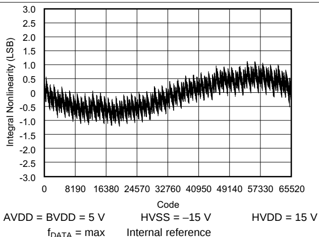
Figure 5. INL vs Code (ADS8556 \pm 10\text{-V}_{IN} Range)
