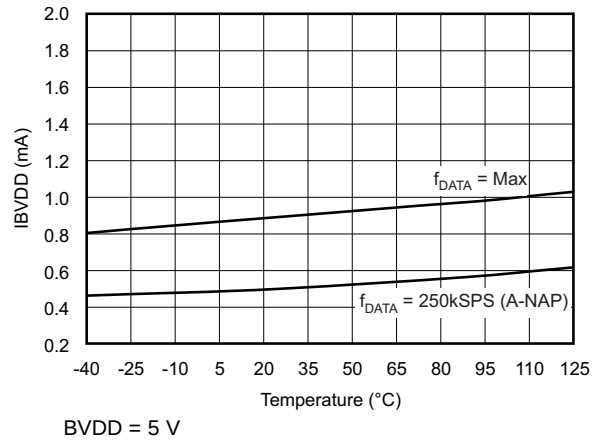
Figure 32. Buffer I/O Supply Current vs Temperature
