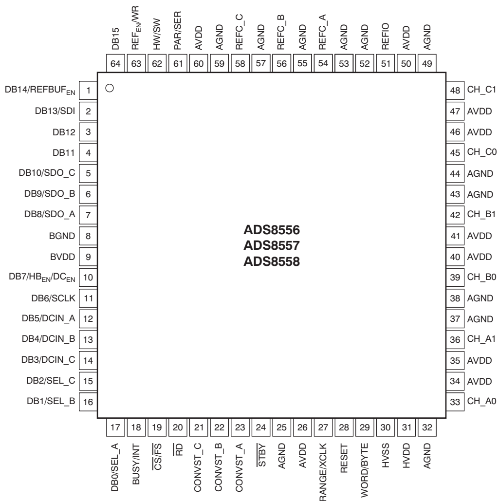
PM Package 64-Pin LQFP Top View
