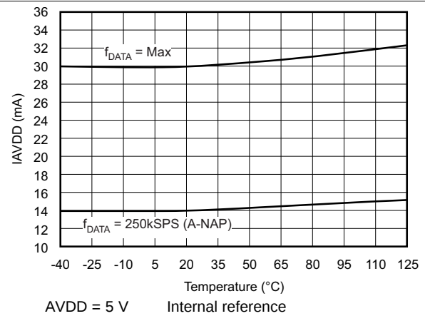
Figure 30. Analog Supply Current vs Temperature
