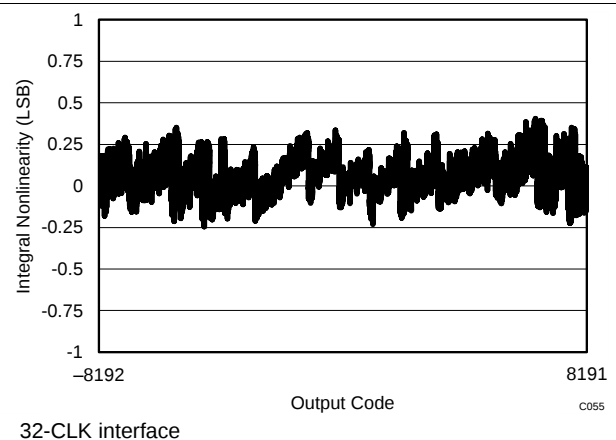
Figure 47. Typical INL
