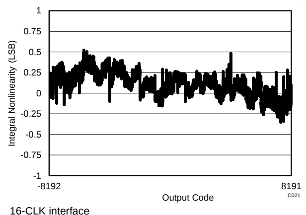
Figure 45. Typical INL
