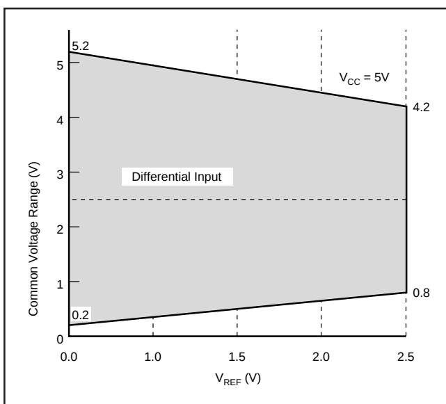
FIGURE 4. Differential Input—Common Voltage Range vs V_{REF} .
