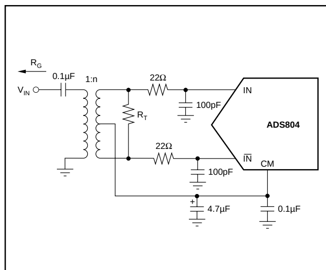
FIGURE 3. Transformer-Coupled Input.
