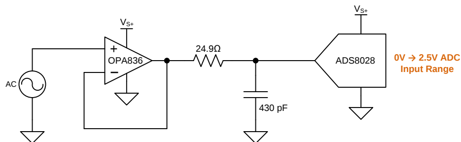
Figure 40. OPA836 Buffer
