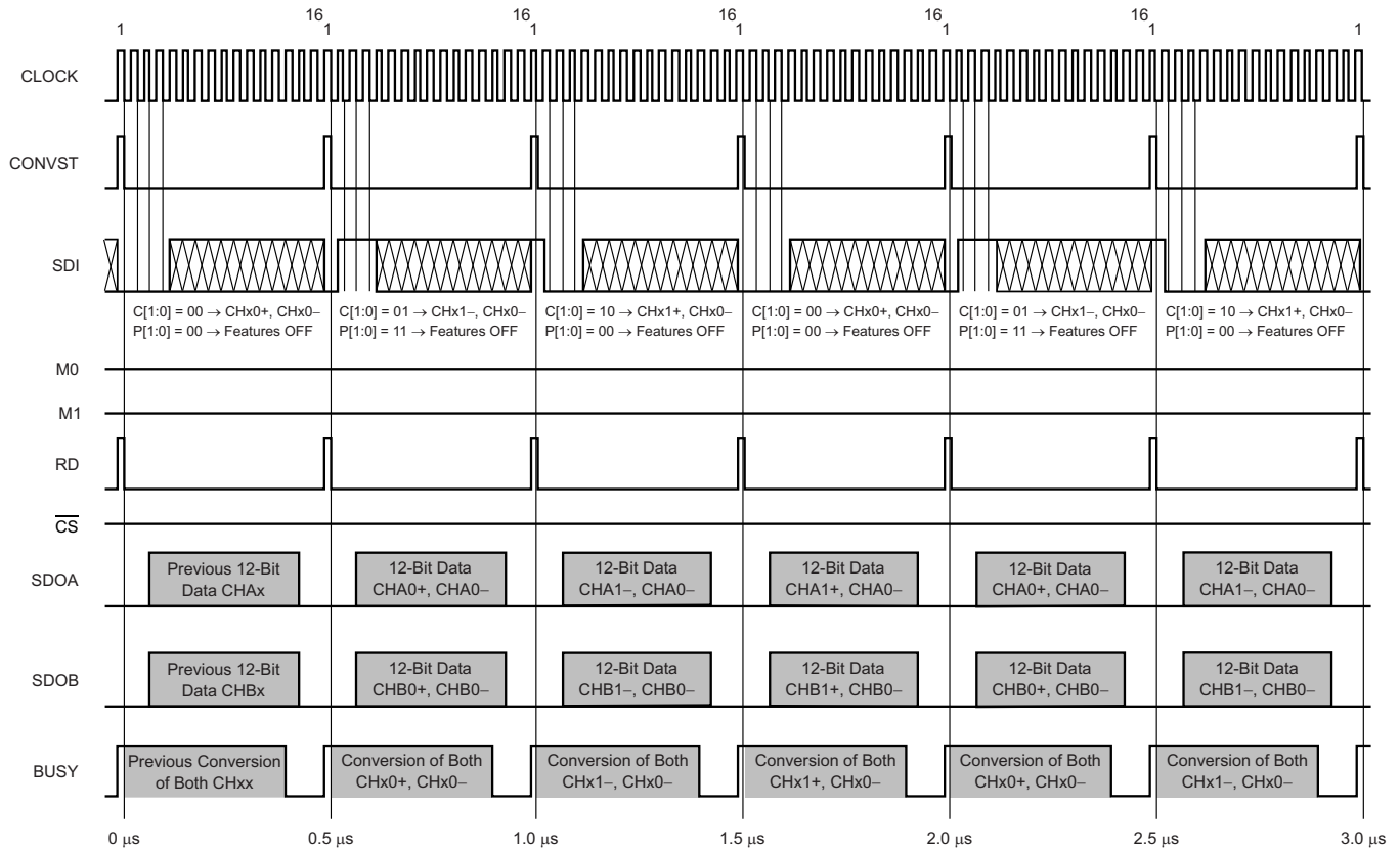
Figure 39. Pseudo-Differential Mode I (M0 = 0, M1 = 0)
