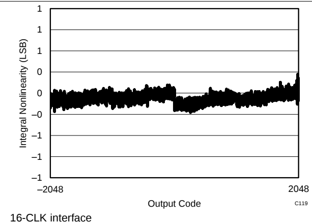
Figure 73. Typical INL
