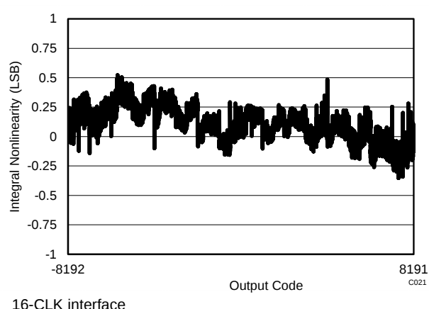
Figure 45. Typical INL
