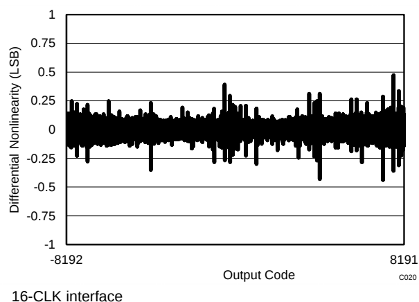
Figure 44. Typical DNL
