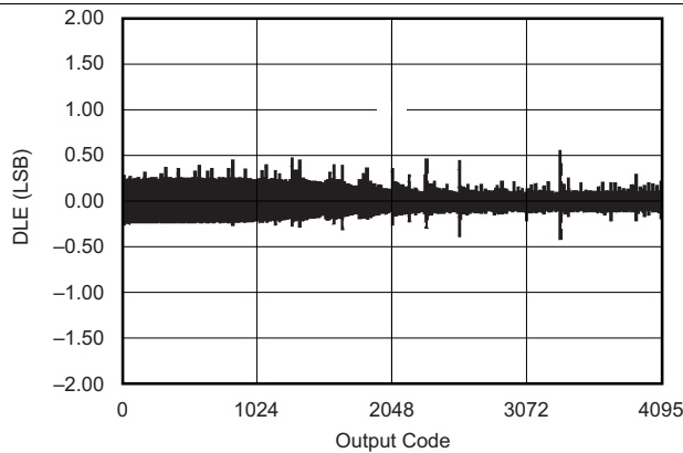
Figure 4. Differential Linearity Error vs Code (2.5-V Internal Reference)
