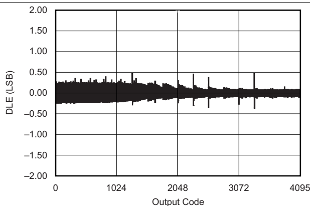
Figure 6. Differential Linearity Error vs Code (2.5-V External Reference)
