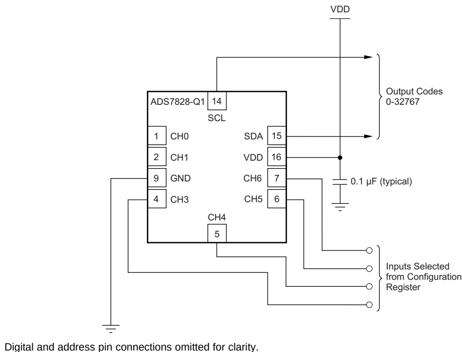
Figure 24. Measuring Single-Ended Inputs
