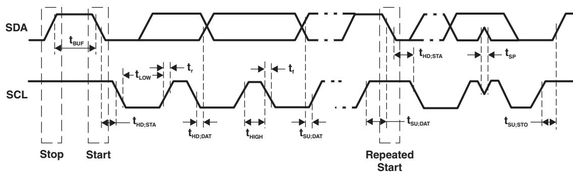
Figure 1. I²C Timing
