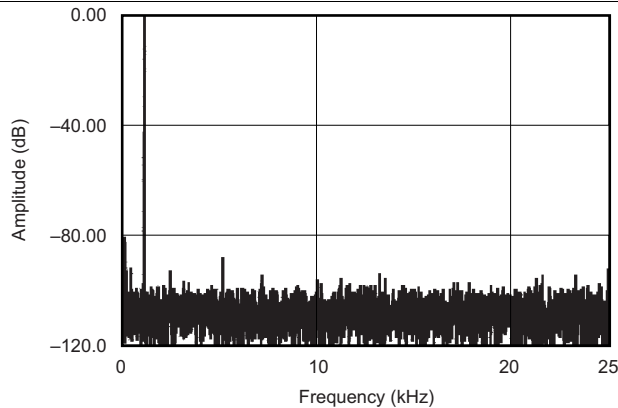
Figure 2. Frequency Spectrum (4096 Point FFT: f_{IN} = 1 kHz, 0 dB)
