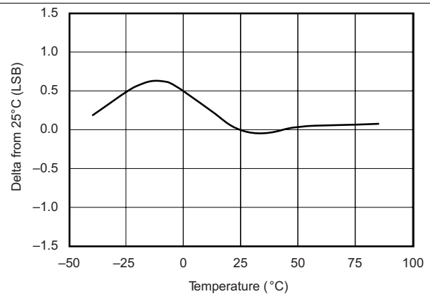
Figure 7. Change in Offset vs Temperature
