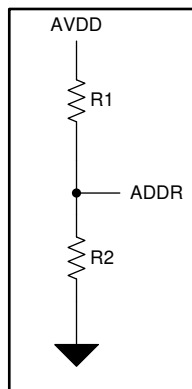
图 7-7. External Resistor Connection Diagram for the ADDR Pin
