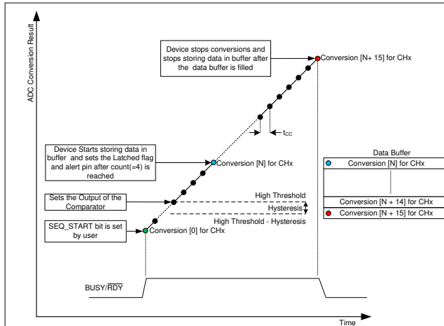
图 7-17. Post- \overline{\text{ALERT}} Data for Single Channel Configurations
