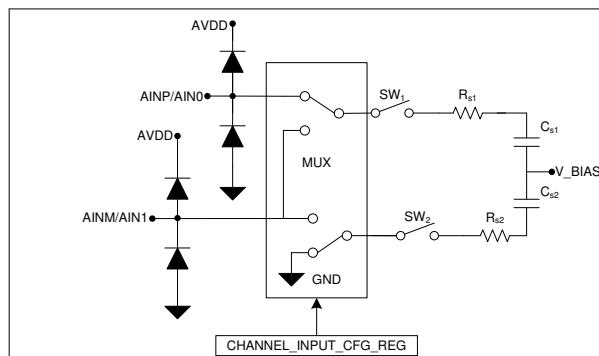
图 7-1. Equivalent Circuit for Analog Input
