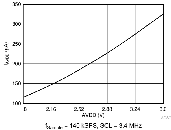
图 6-25. I_{AVDD} in Manual Mode vs AVDD
