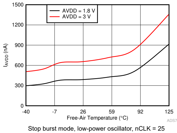
图 6-31. I_{AVDD} in Autonomous Modes vs Temperature
