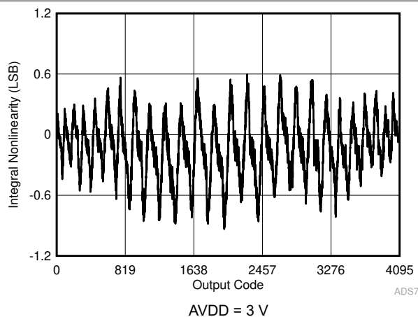
图 6-19. Typical INL in Manual Mode
