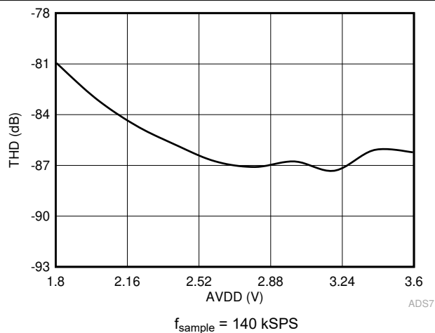
图 6-11. THD in Manual Mode vs AVDD
