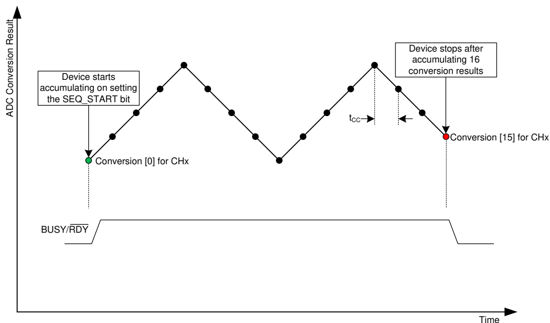
图 7-24. High-Precision Mode With Single-Channel Configurations
