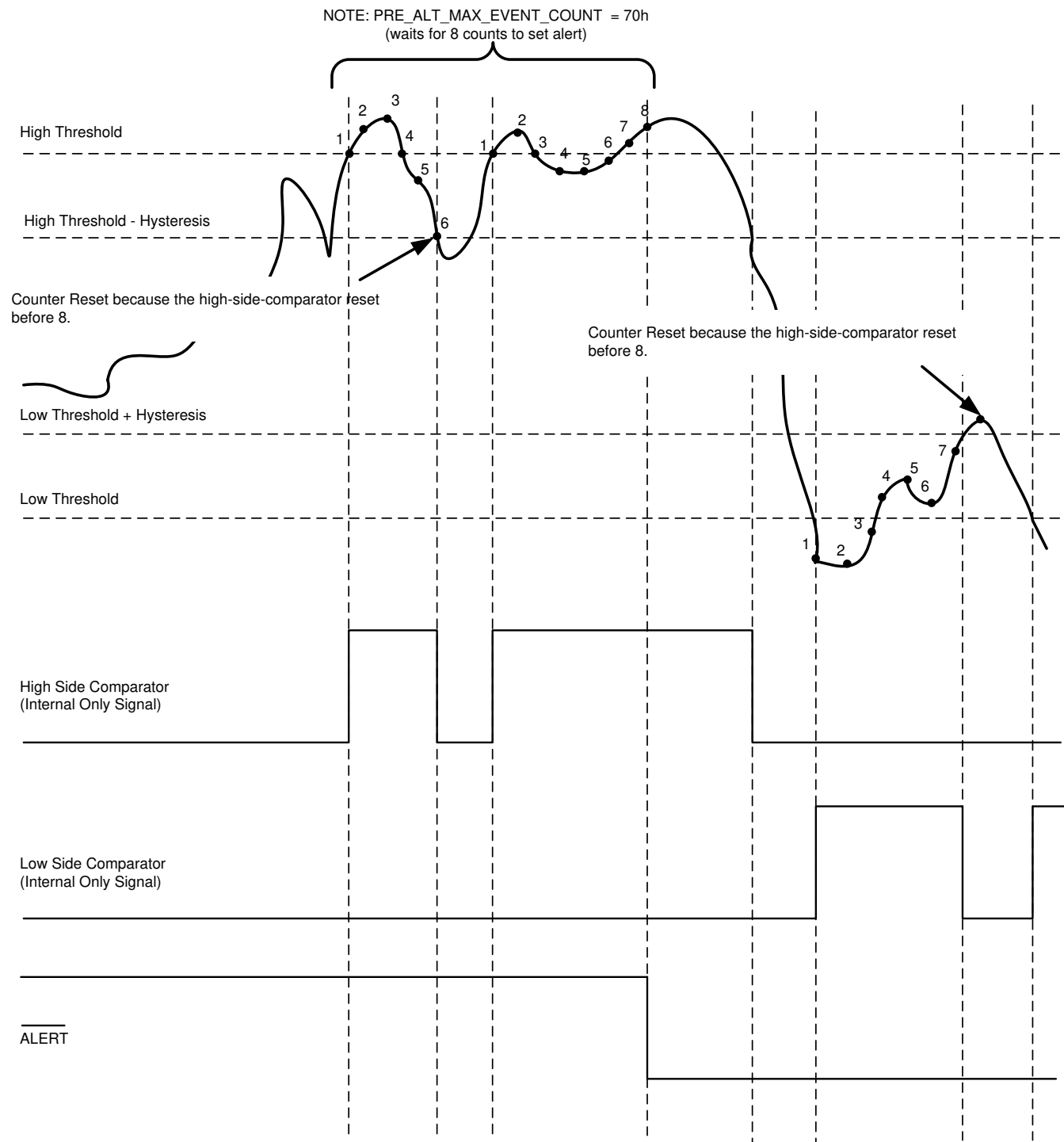
图 7-10. Thresholds, Hysteresis, and Event Counter for the Digital Window Comparator
