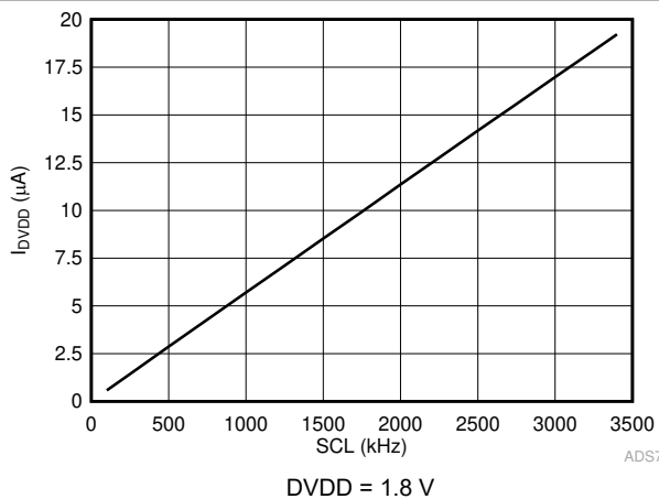
图 6-27. I_{DVDD} in Manual Mode vs SCL
