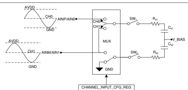
图 7-2. Two-Channel, Single-Ended Configuration
