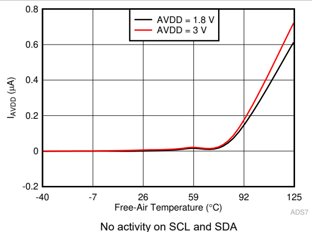
图 6-28. Static I_{AVDD} in Manual Mode vs Temperature
