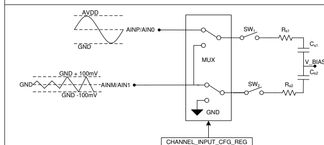
图 7-3. Single-Channel, Single-Ended Configuration With Remote Ground Sensing
