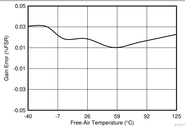
图 6-15. Gain Error in Manual Mode vs Free-Air Temperature
