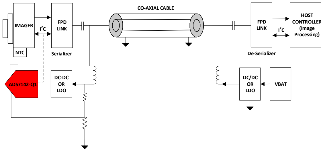
图 8-8. Voltage and Temperature Sensing in Remote Camera Modules Using the ADS7142-Q1
