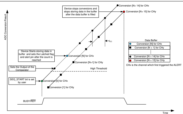
图 7-18. Post- \overline{\text{ALERT}} Data for Dual Channel Configuration
