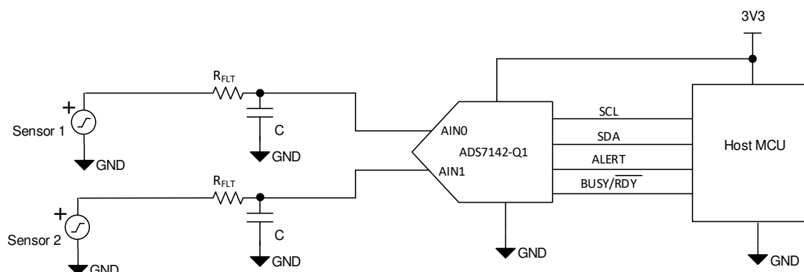
图 8-2. Sensor Monitor Circuit With the ADS7142-Q1
