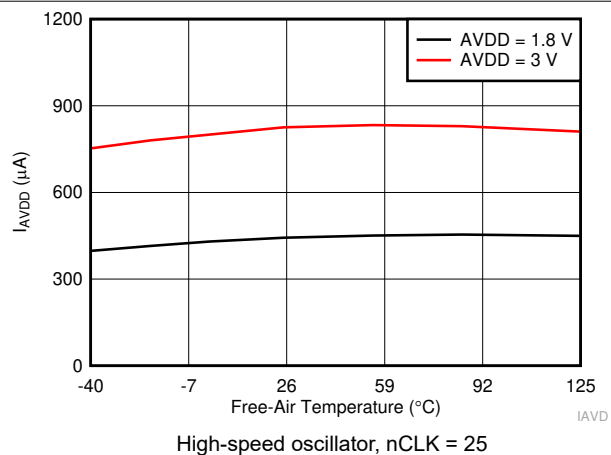
图 6-36. I_{AVDD} in High-Precision Mode vs Temperature
