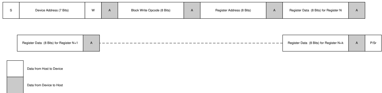
图 7-30. Writing a Continuous Block of Registers
