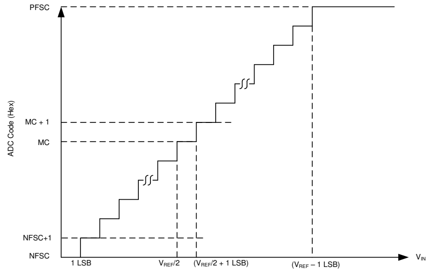
图 7-5. Ideal Transfer Characteristics for Single-Ended Configurations
