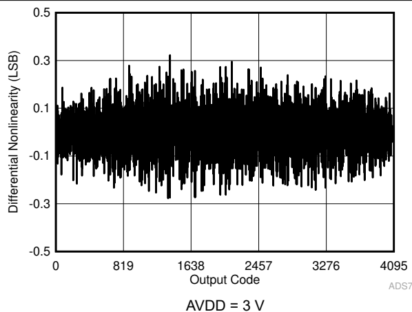
图 6-17. Typical DNL in Manual Mode
