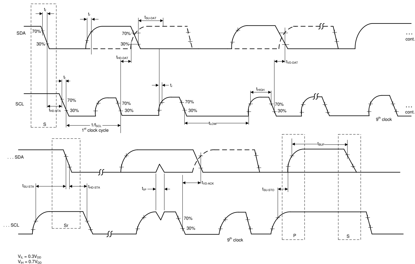
图 6-1. Timing Diagram for Standard Mode, Fast Mode, and Fast Mode Plus
