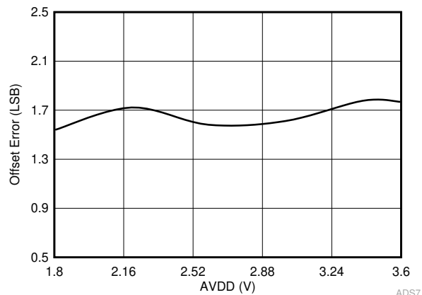
图 6-14. Offset Error in Manual Mode vs AVDD
