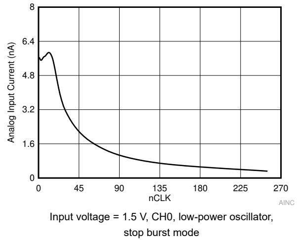
图 6-30. Analog Input Current in Autonomous Modes vs nCLK
