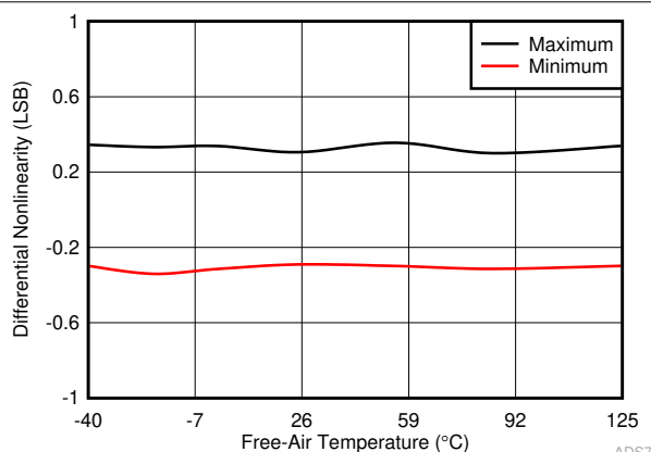
图 6-21. DNL in Manual Mode vs Temperature
