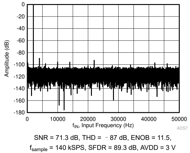
图 6-6. Typical FFT in Manual Mode
