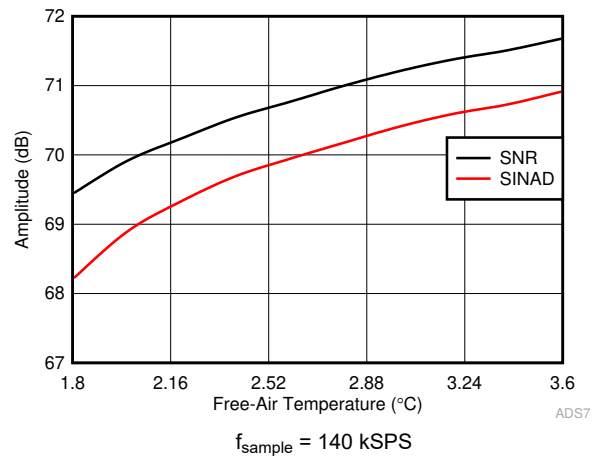
图 6-8. SNR and SINAD in Manual Mode vs AVDD
