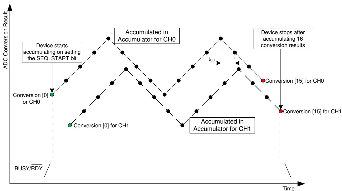
图 7-25. High-Precision Mode With Dual-Channel Configurations
