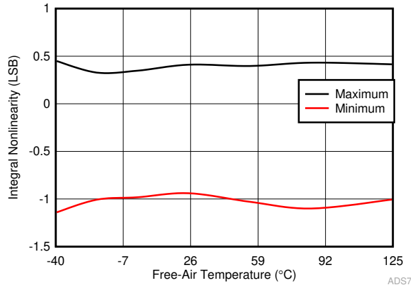
图 6-23. INL in Manual Mode vs Temperature
