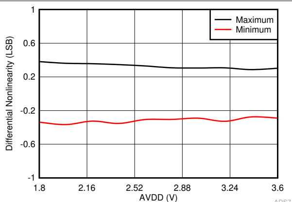
图 6-22. DNL in Manual Mode vs AVDD
