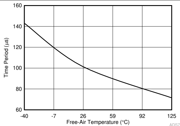
图 6-4. Low-Power Oscillator Time Period vs Temperature
