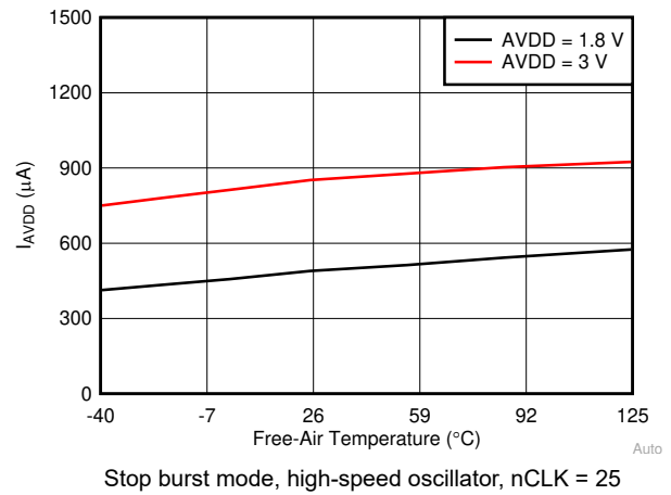
图 6-32. I_{AVDD} in Autonomous Modes vs Temperature
