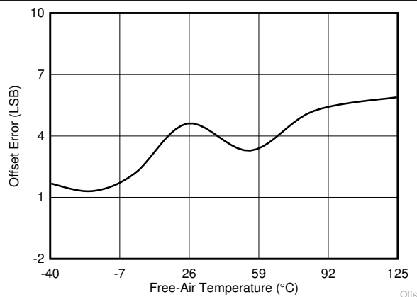
图 6-33. Offset Error in High-Precision Mode vs Temperature
