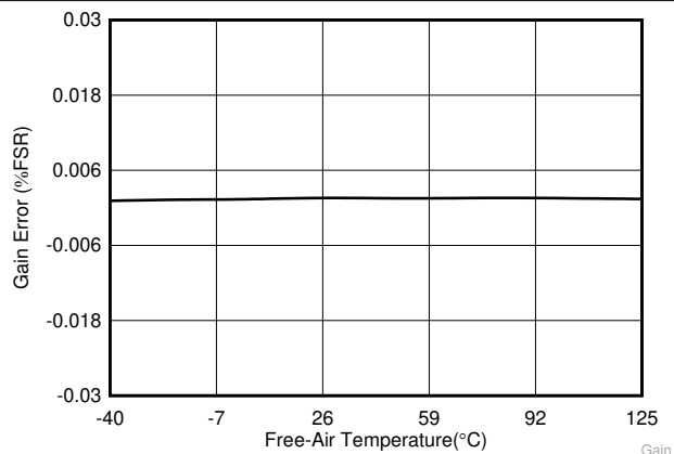
图 6-34. Gain Error in High-Precision Mode vs Temperature
