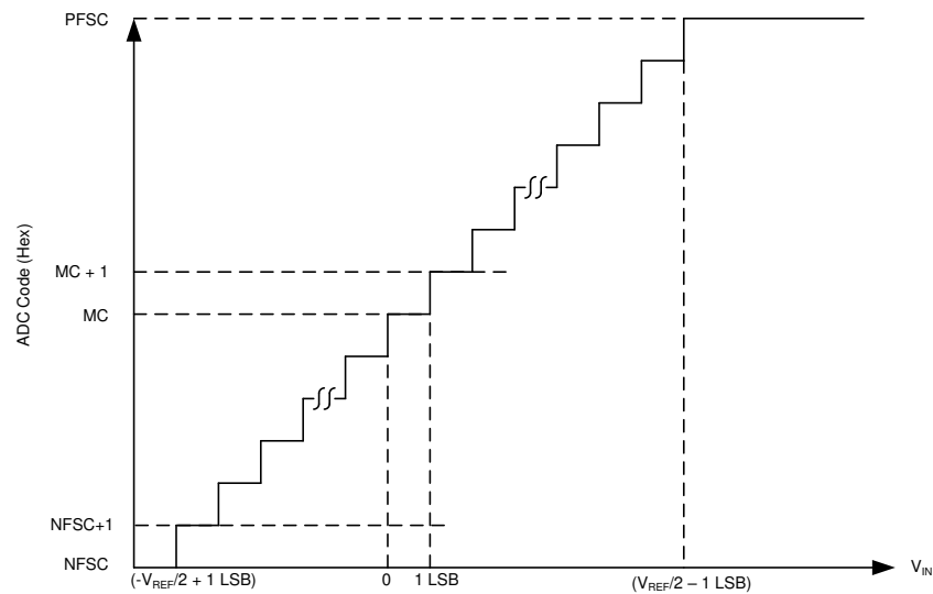
图 7-6. Ideal Transfer Characteristics for Pseudo-Differential Configuration
