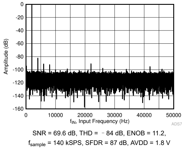
图 6-5. Typical FFT in Manual Mode
