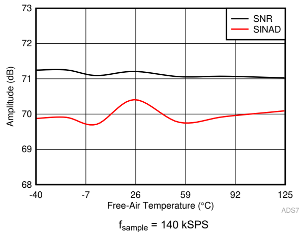
图 6-7. SNR and SINAD in Manual Mode vs Temperature
