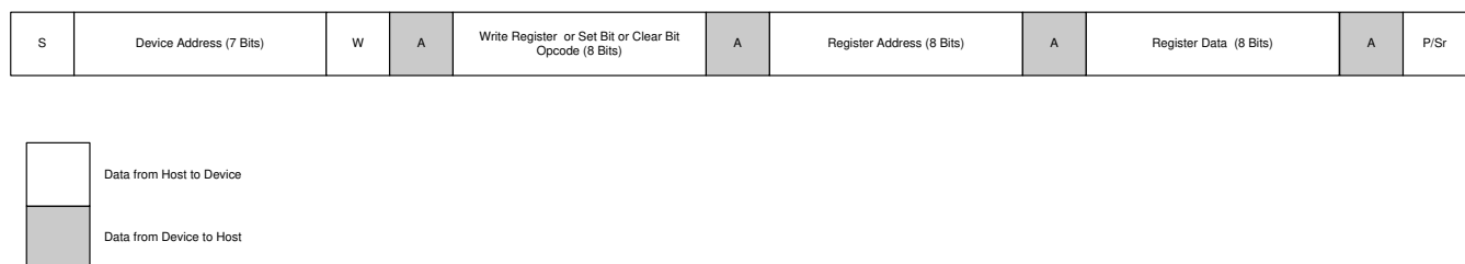
图 7-29. Writing a Single Register
