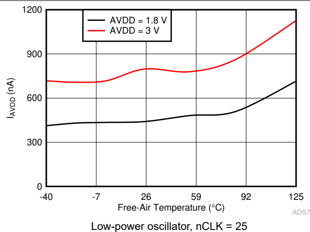
图 6-35. I_{AVDD} in High-Precision Mode vs Temperature
