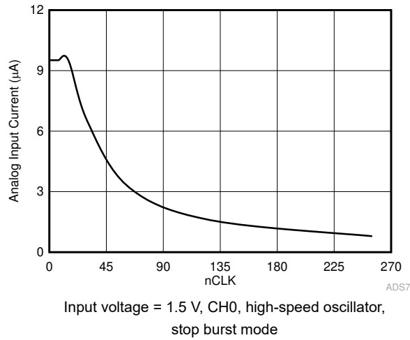
图 6-29. Analog Input Current in Autonomous Modes vs nCLK
