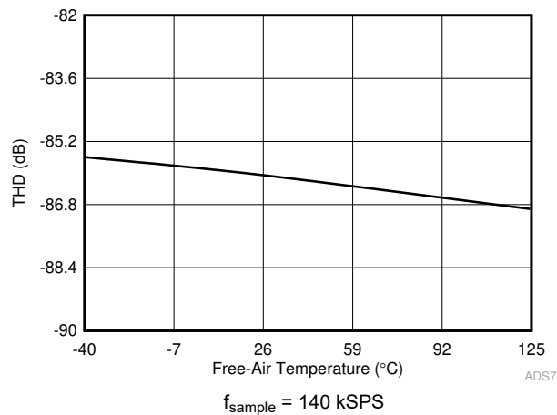
图 6-9. THD in Manual Mode vs Temperature
