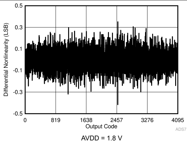
图 6-18. Typical DNL in Manual Mode
