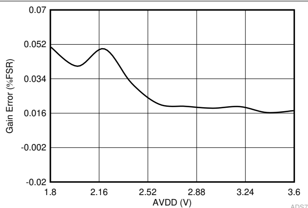
图 6-16. Gain Error in Manual Mode vs AVDD
