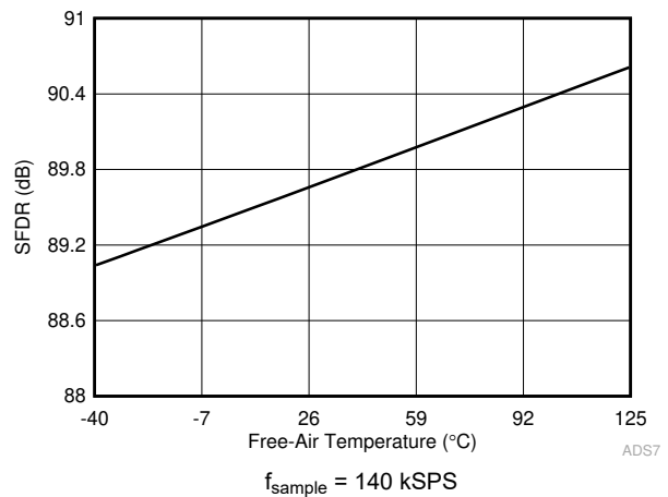
图 6-10. SFDR in Manual Mode vs Temperature
