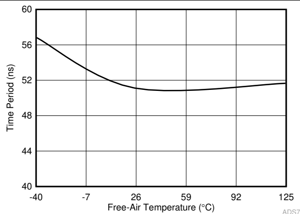
图 6-3. High-Speed Oscillator Time Period vs Temperature
