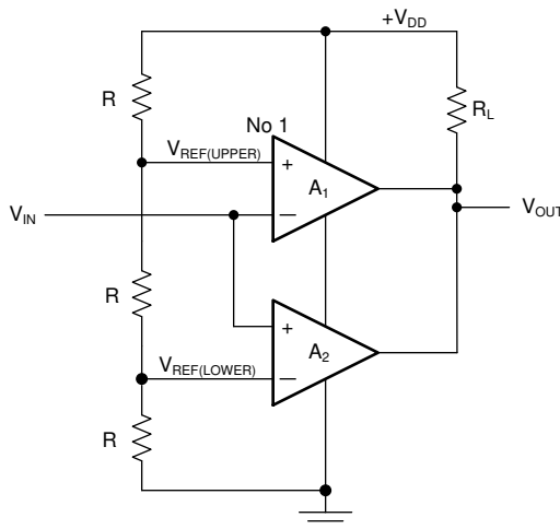
图 8-1. Analog Window Comparator
