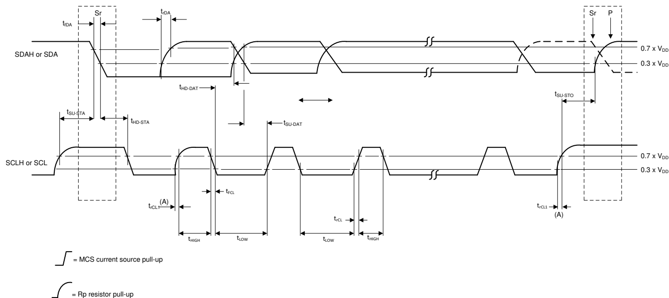
图 6-1. Timing Diagram for Standard Mode, Fast Mode, and Fast Mode Plus
