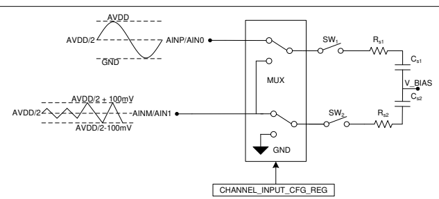
图 7-4. Single-Channel, Pseudo-Differential Configuration
