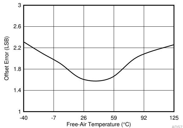
图 6-13. Offset Error in Manual Mode vs Temperature
