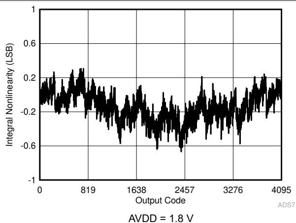
图 6-20. Typical INL in Manual Mode
