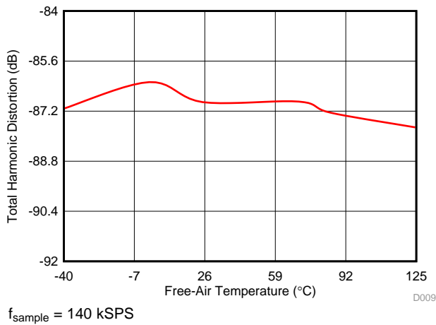
图 9. THD in Manual Mode with Temperature
