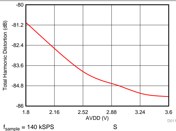
图 11. THD in Manual Mode with AVDD
