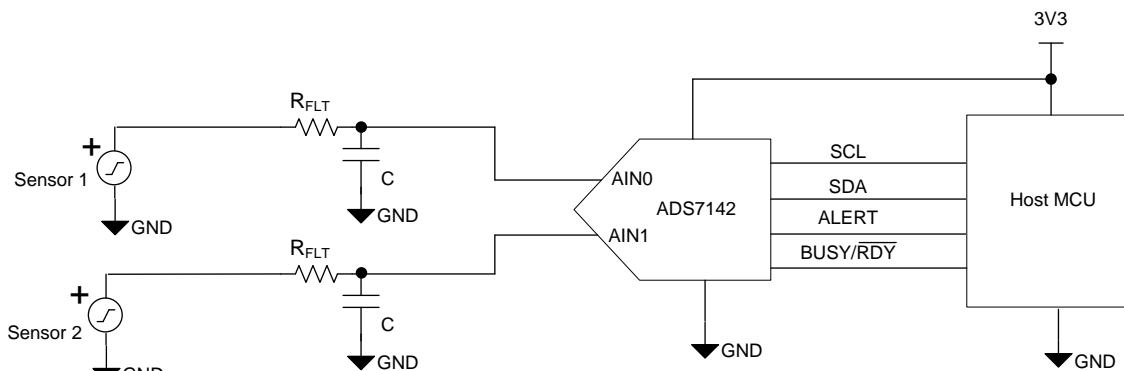
图 113. Sensor Monitor Circuit with ADS7142
