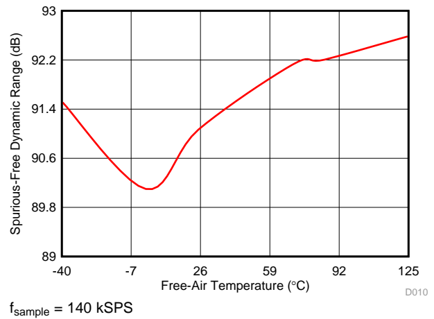
图 10. SFDR in Manual Mode with Temperature
