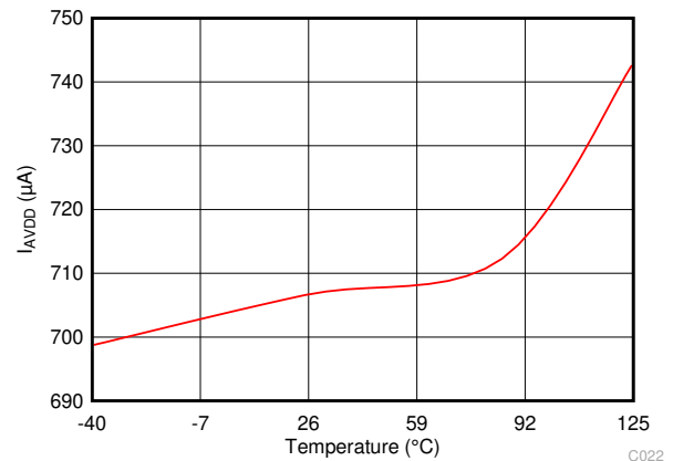
图 7-23. Analog Supply Current vs Temperature (OSC_SEL = 0, CLK_DIV = 0) in Turbo Comparator Mode
