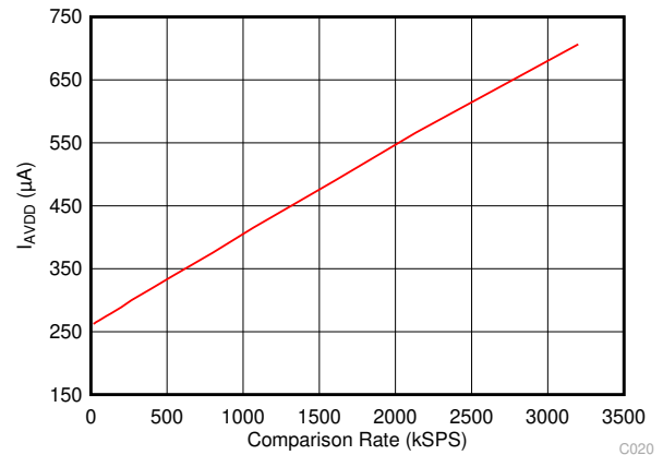
图 7-21. Analog Supply Current vs Comparison Rate (OSC_SEL = 0) in Turbo Comparator Mode
