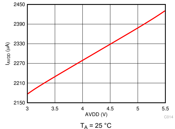
图 5-20. Analog Supply Current vs AVDD
