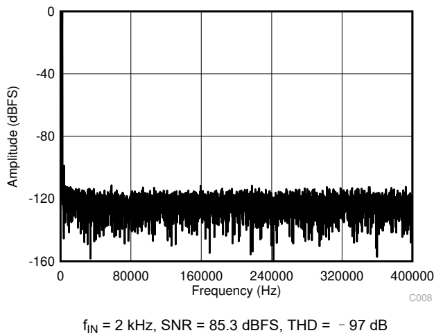
图 7-2. Test Results for the Single-Supply DAQ Circuit
