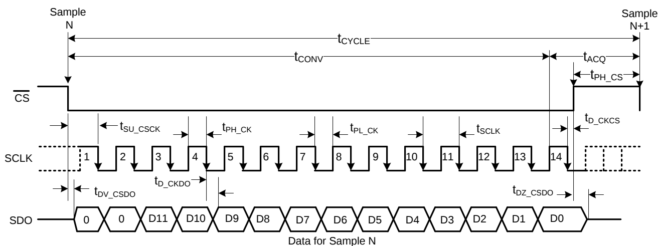
Figure 1. Timing Diagram
