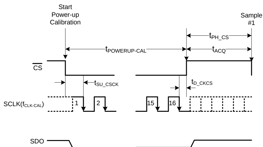
Figure 38. Offset Calibration on Power-Up Timing Diagram
