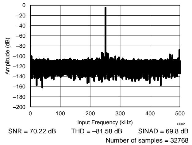
Figure 43. Test Results for the ADS7042 and OPA835 for a 250-kHz Input
