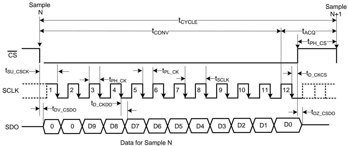
Figure 1. Timing Diagram
