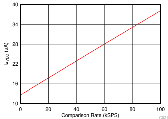
图 7-21. Analog Supply Current vs Throughput
