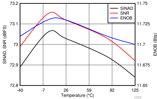
图 6-15. Noise Performance vs Temperature
