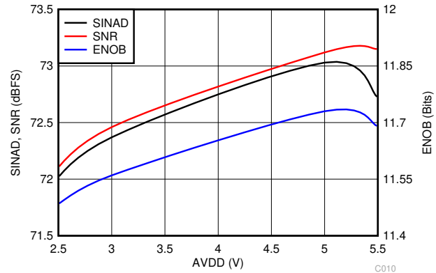
图 6-16. Noise Performance vs AVDD
