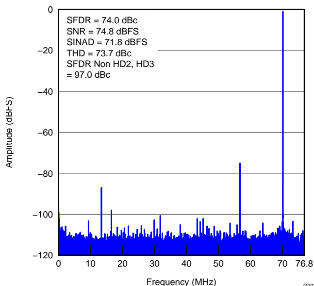
Figure 9. AMPLITUDE vs FREQUENCY (70-MHz IF)
