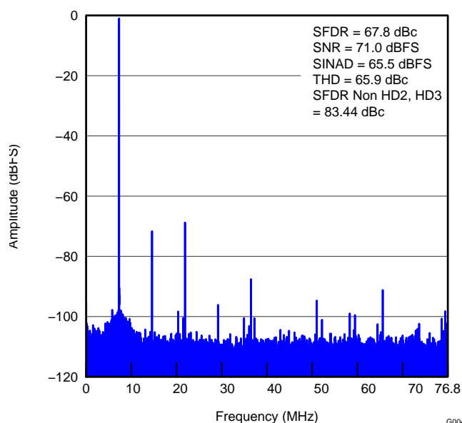
Figure 11. AMPLITUDE vs FREQUENCY (300-MHz IF)
