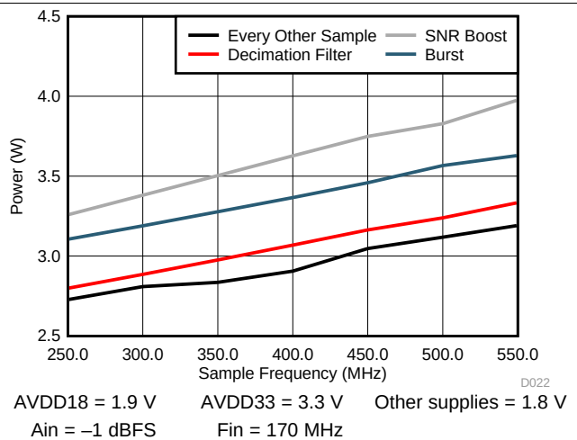
图 27. Power vs. Sample Frequency
