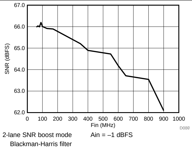
图 35. SNR Boost SNR vs Frequency
