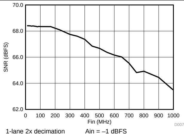
图 11. SNR vs. Frequency
