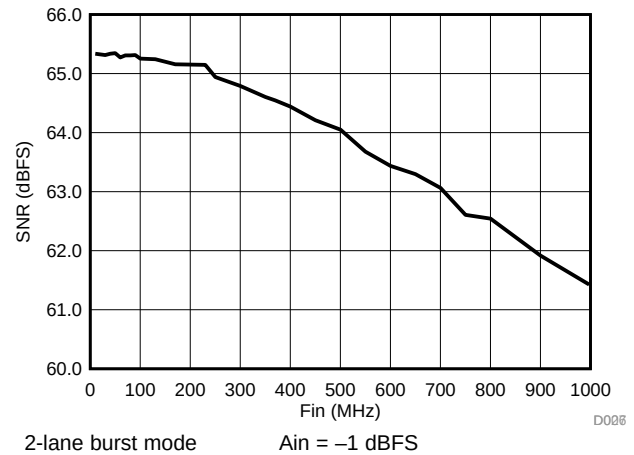
图 31. Burst Mode SNR vs Frequency
