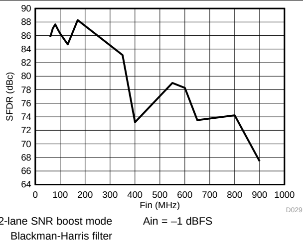
图 34. SNR Boost SFDR vs. Frequency
