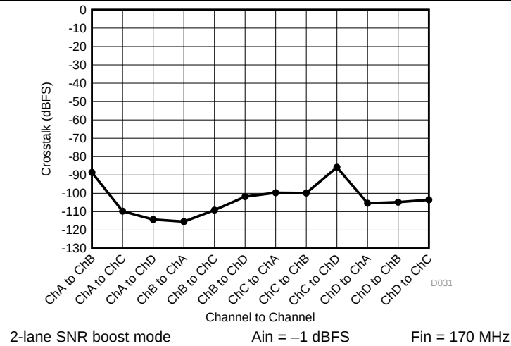
图 36. SNR Boost Crosstalk by Channel
