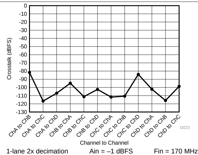
图 28. Crosstalk by Channel
