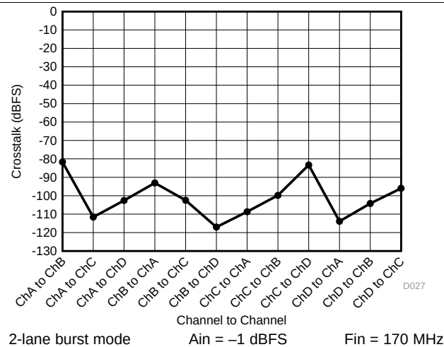
图 32. Burst Mode Crosstalk by Channel
