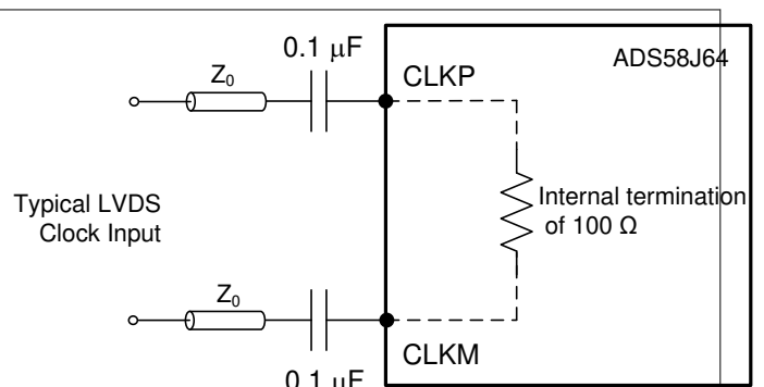
图 7-3. LVDS Clock Driving Circuit
