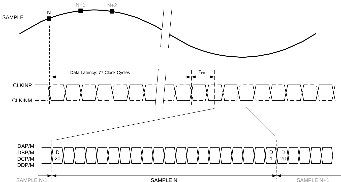
Figure 1. Latency Timing Diagram
