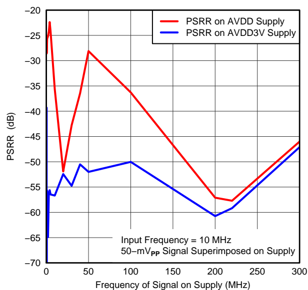
Figure 35. POWER-SUPPLY REJECTION RATIO vs FREQUENCY
