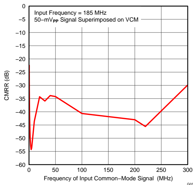
Figure 33. COMMON-MODE REJECTION RATIO vs FREQUENCY
