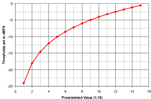
图 8-6. OVR Detection Threshold
