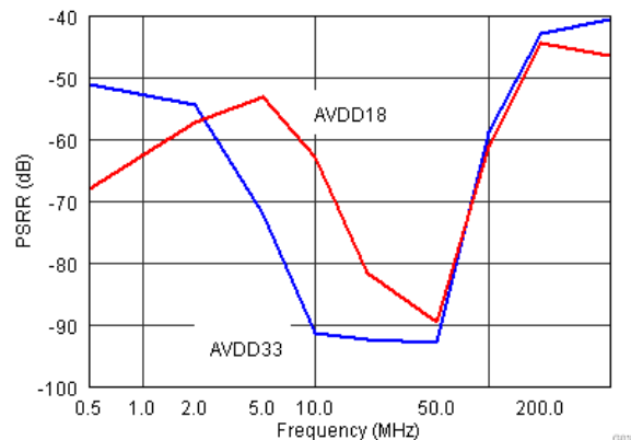
图 7-27. PSRR Across Frequency
