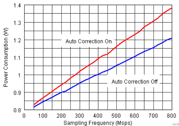
图 7-28. Power Across Sampling Frequency
