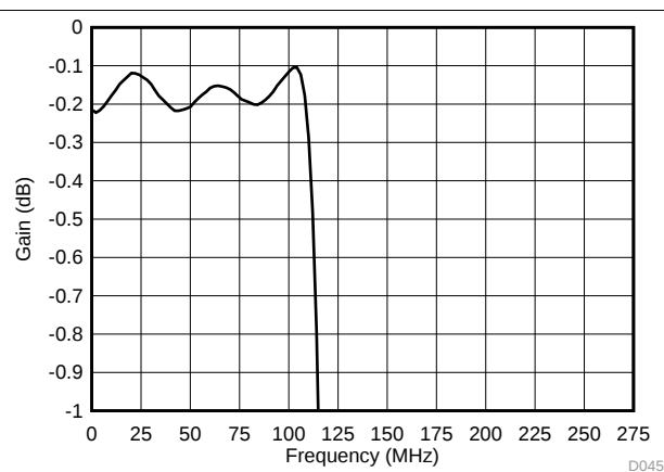
图 53. Decimation Filter Pass-Band Ripple vs Frequency
