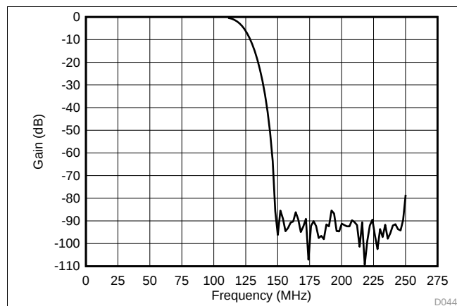
图 52. Decimation Filter Response vs Frequency
