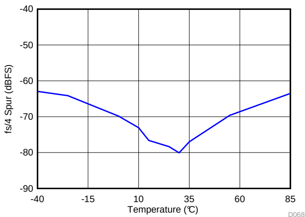
Figure 144. Variation of the f_s / 4 Spur Over Temperature
