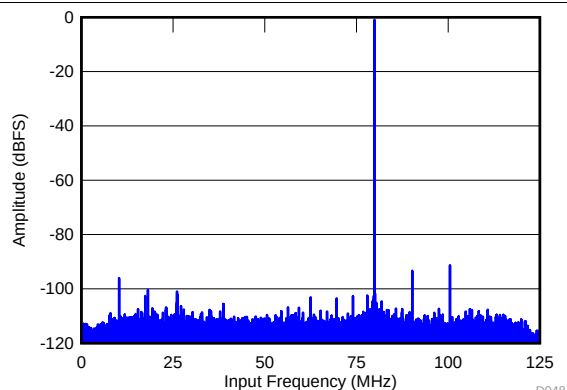
SNR = 75.2 dBFS, SFDR = 90 dBc Figure 51. FFT for 170-MHz Input Signal in Decimate-by-4 Mode
