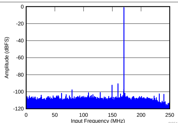
SNR = 71.9 dBFS, SFDR = 89 dBc Figure 54. FFT for 170-MHz Input Signal in Decimate-by-2 Mode
