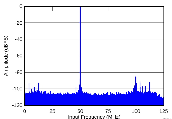
SNR = 69.6 dBFS, SFDR = 84 dBc Figure 53. FFT for 450-MHz Input Signal in Decimate-by-4 Mode
