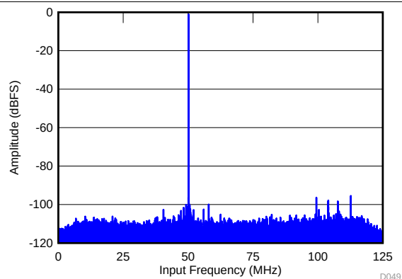
SNR = 72.8 dBFS, SFDR = 91 dBc Figure 52. FFT for 300-MHz Input Signal in Decimate-by-4 Mode
