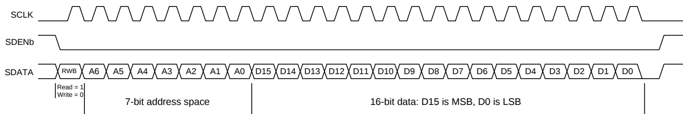
图 71. Serial Register Read Timing Diagram
