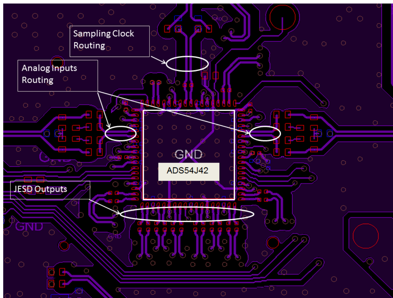
Figure 139. ADS54J42EVM Layout
