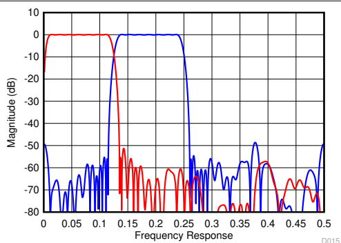
图 8-6. Decimate-by-4 Filter Response
