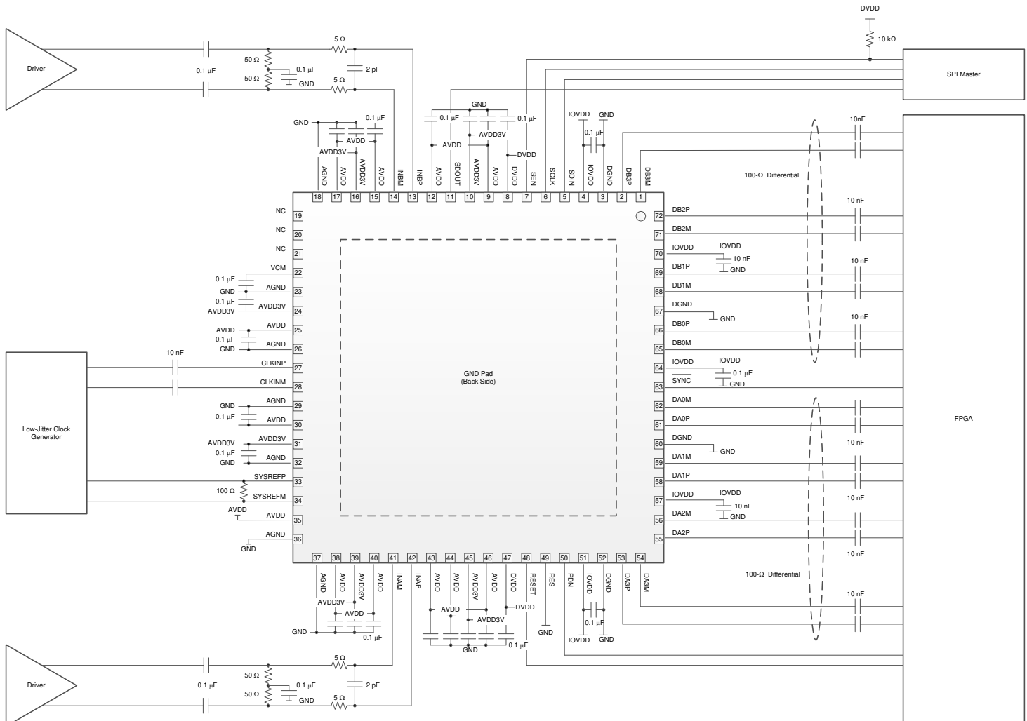
图 9-14. AC-Coupled Receiver
