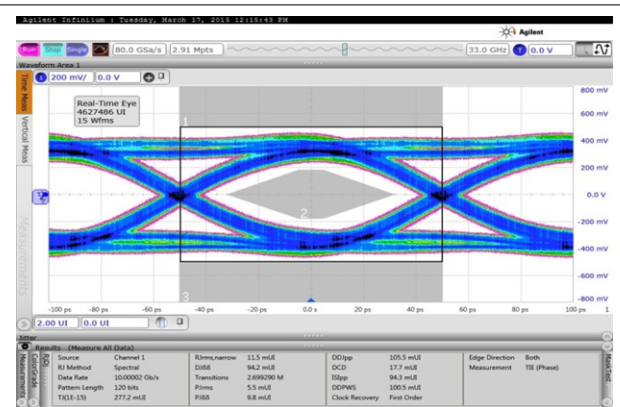
图 8-26. Eye at 10-Gbps Bit Rate with Increased Output Swing
