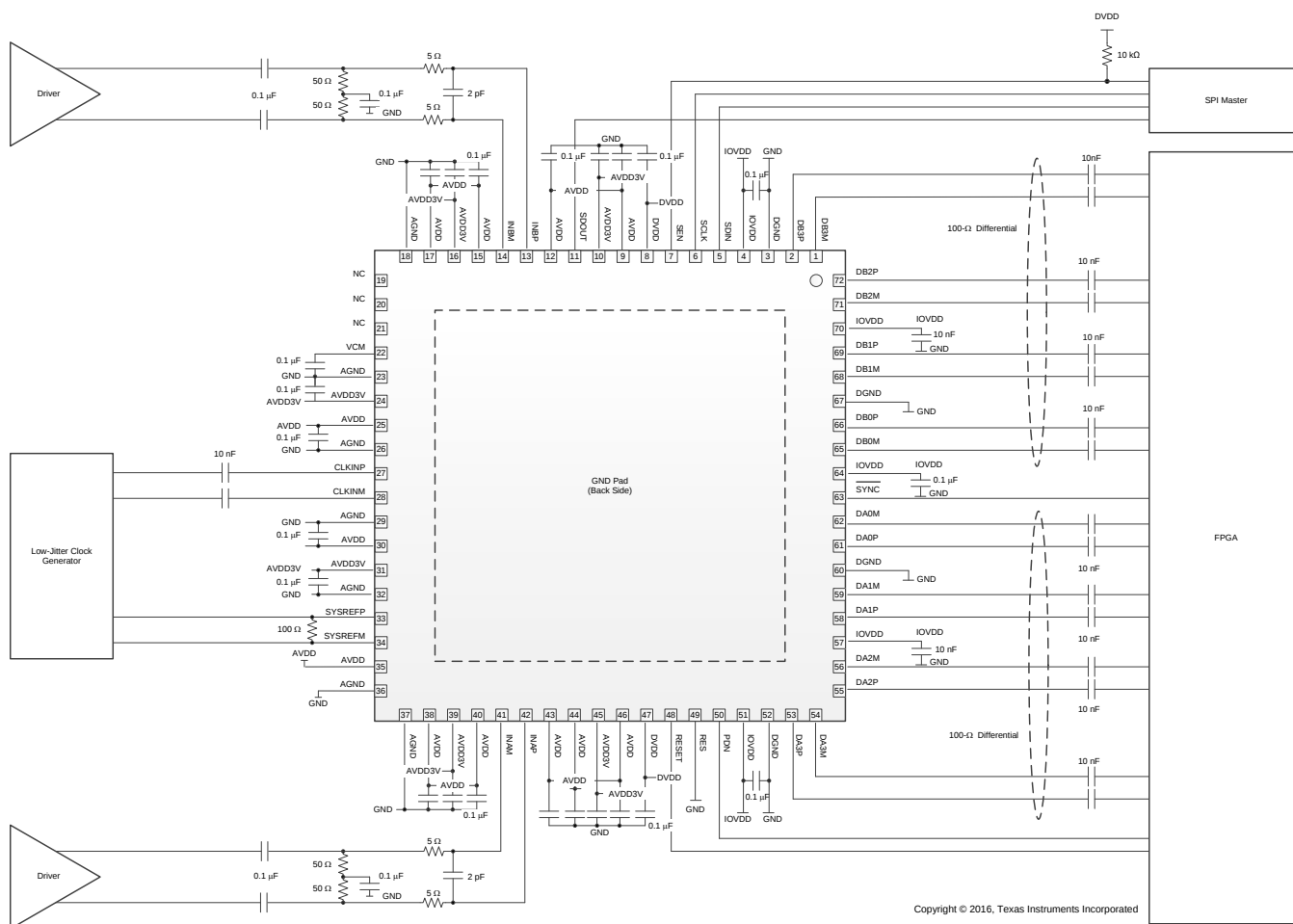
Figure 132. AC-Coupled Receiver
