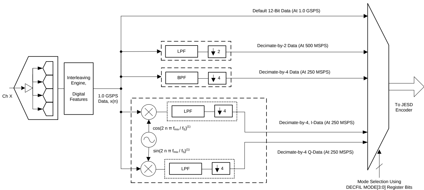
Figure 59. DDC Block
