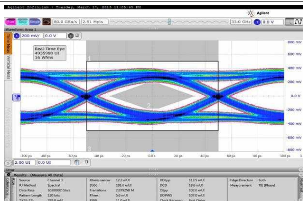
Figure 80. Eye Diagram at 10-Gbps Bit Rate with Default Output Swing
