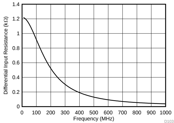
Figure 133. R_{IN} vs Input Frequency
