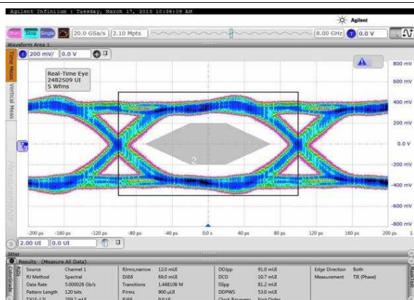
Figure 78. Eye Diagram at 5-Gbps Bit Rate with Default Output Swing
