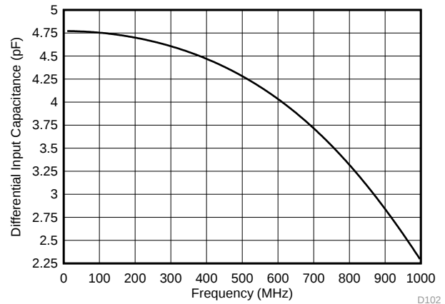
Figure 134. C_{IN} vs Input Frequency
