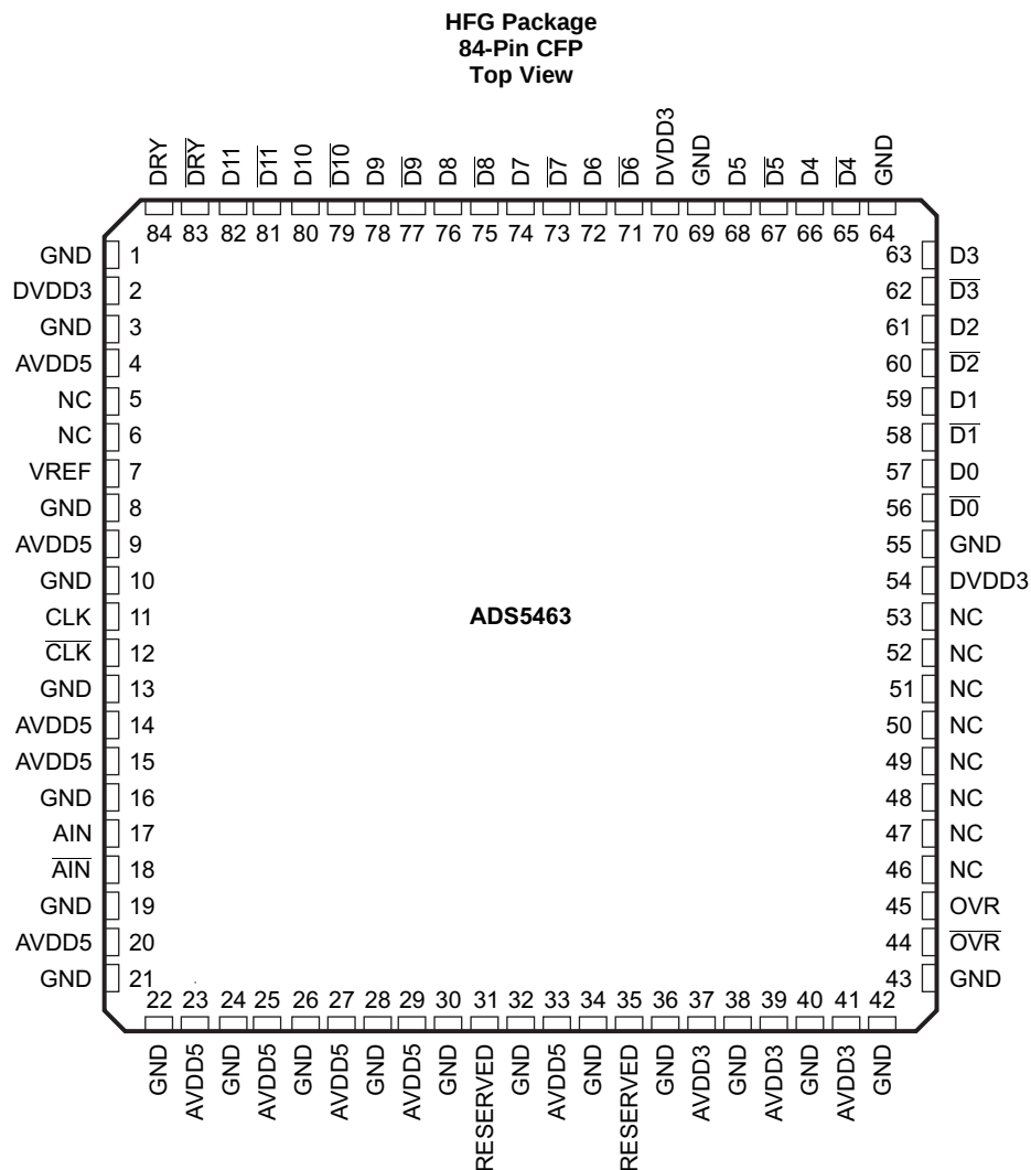
Pin Functions
