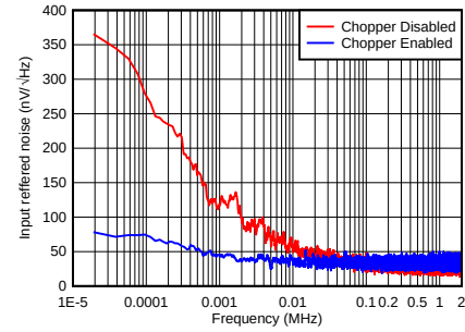
图 39. Low-Frequency Noise With and Without Chopper Enabled
