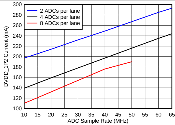
图 46. DVDD_1P2 Current vs ADC Sample Rate
