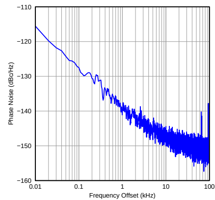
图 25. Phase Noise for 5-MHz Input Signal, Sample Rate = 80 MSPS
