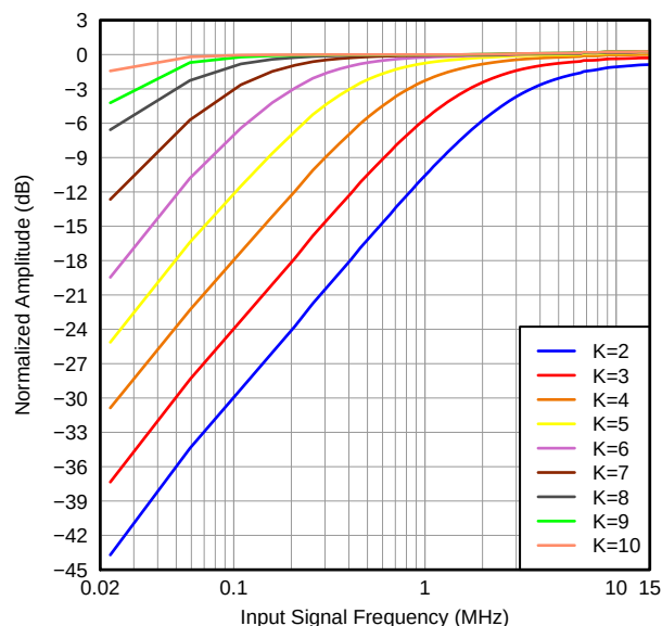
图 47. HP Filter Amplitude Response at K = 2 to 10
