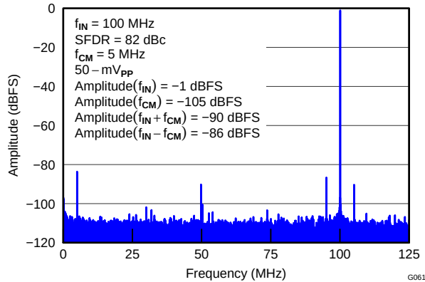
Figure 61. CMRR FFT
