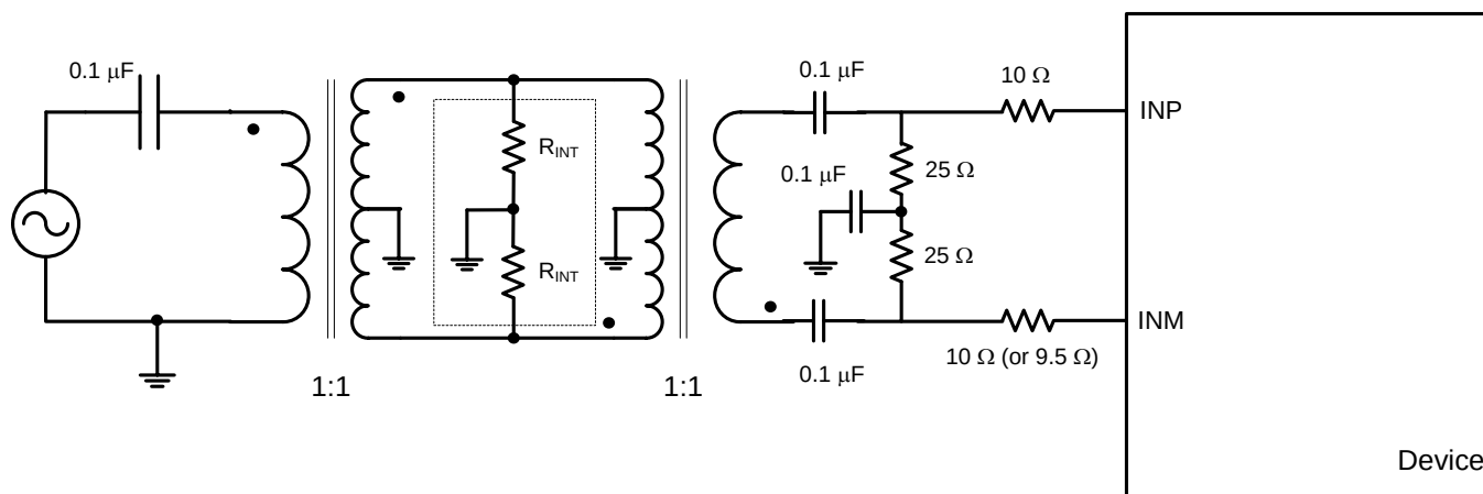
Figure 114. Drive Circuit for Input Frequencies > 250 MHz
