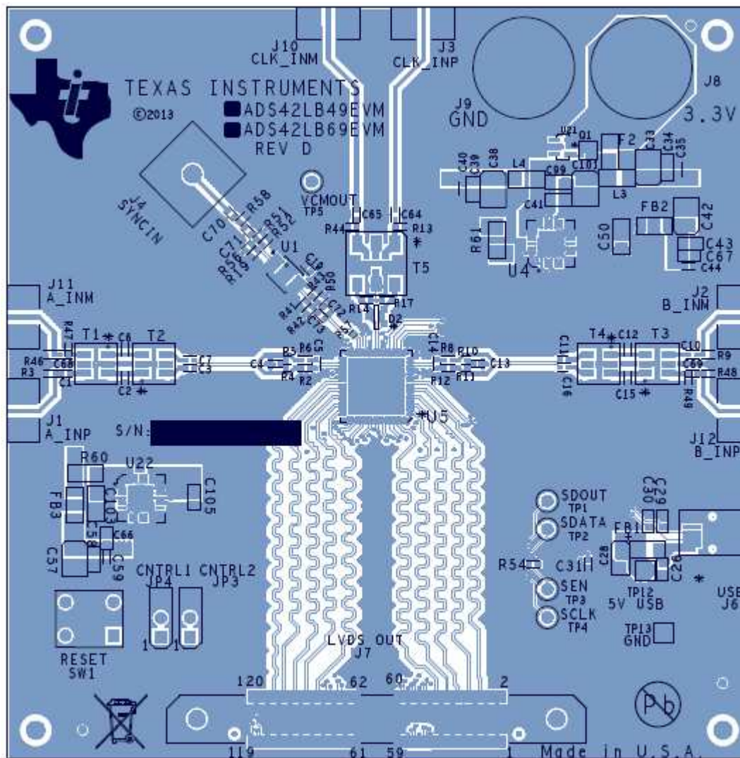
Figure 127. Example Layout
