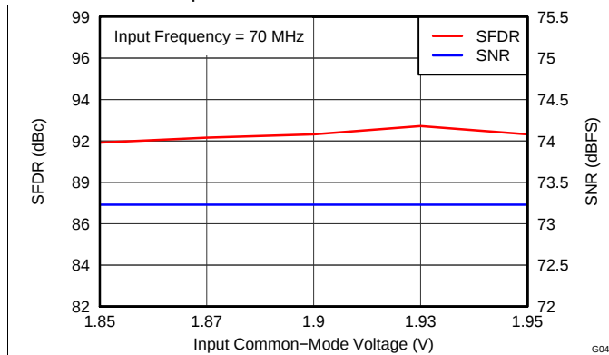
Figure 50. Performance vs Input Common-Mode Voltage (70 MHz)
