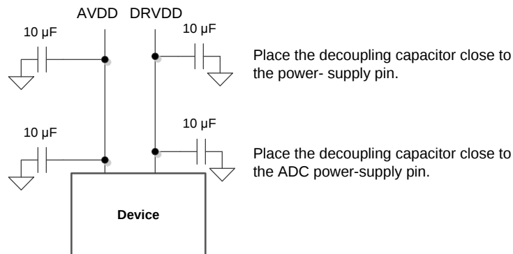
Figure 125. Recommended Placement of Power-Supply Decoupling Capacitors
