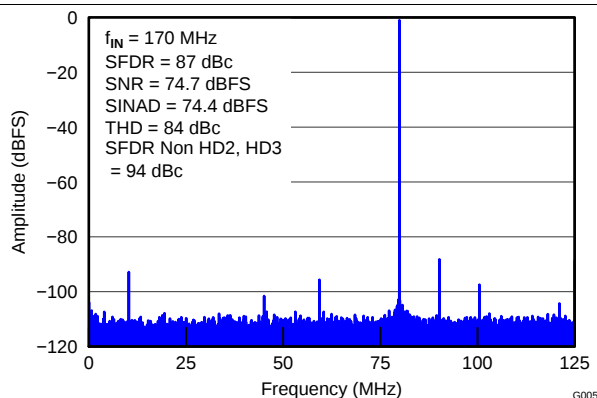
Figure 6. FFT for 170-MHz Input Signal (2.5- V_{\text{PP}} Full-Scale)
