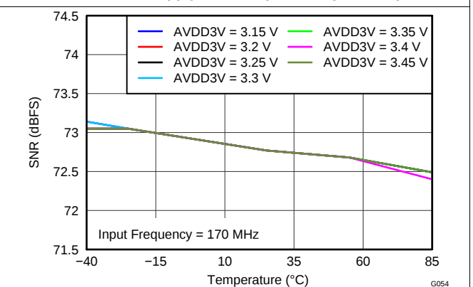
Figure 53. Signal-to-Noise Ratio vs AVDD Supply and Temperature (170 MHz)
