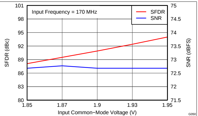
Figure 51. Performance vs Input Common-Mode Voltage (170 MHz)
