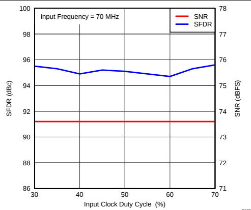
图 34. Performance vs Clock Duty Cycle (70 MHz)
