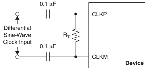
图 81. Differential Sine-Wave Clock Driving Circuit
