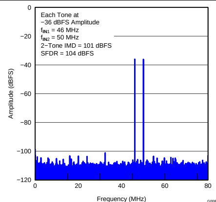
图 13. FFT for Two-Tone Input Signal ( -36\text{ dBFS} at 46 MHz and 50 MHz)
