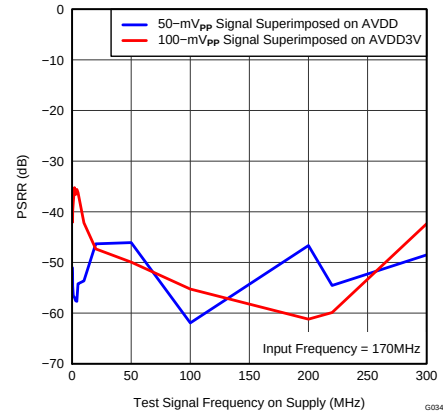
图 39. Power-Supply Rejection Ratio vs Test Signal Frequency
