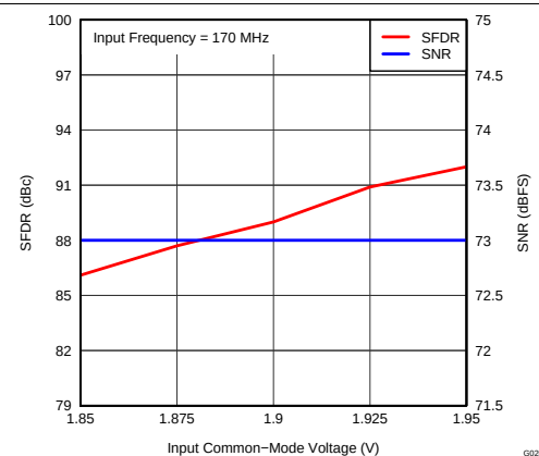
图 25. Performance vs Input Common-Mode Voltage (170 MHz)
