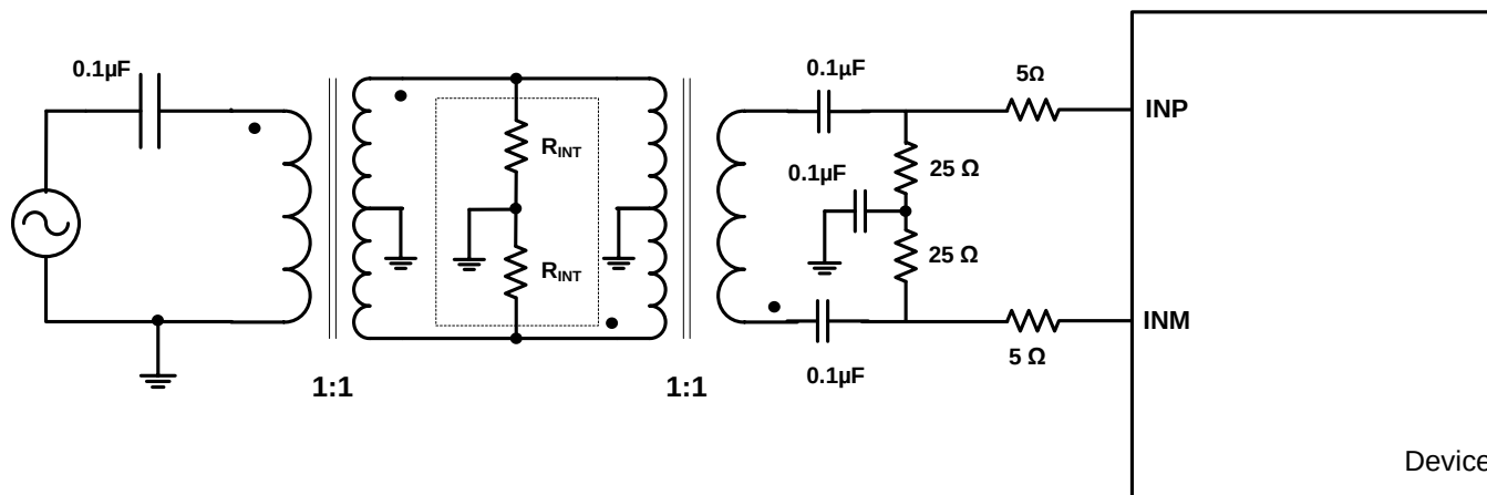
图 80. Drive Circuit for Input Frequencies > 250 MHz
