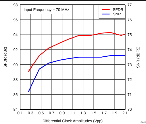
图 32. Performance vs Clock Amplitude (70 MHz)
