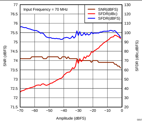
图 22. Performance vs Input Amplitude (70 MHz)
