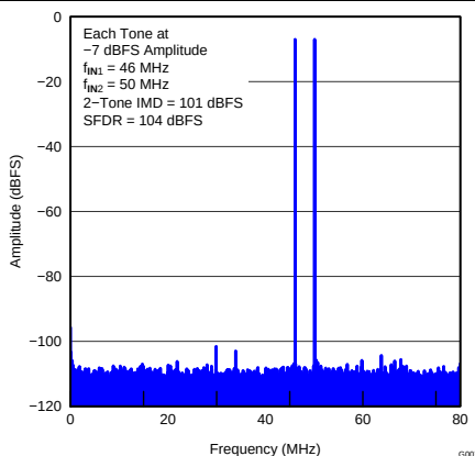
图 12. FFT for Two-Tone Input Signal ( -7\text{ dBFS} at 46 MHz and 50 MHz)
