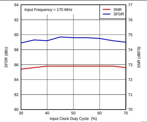
图 35. Performance vs Clock Duty Cycle (170 MHz)
