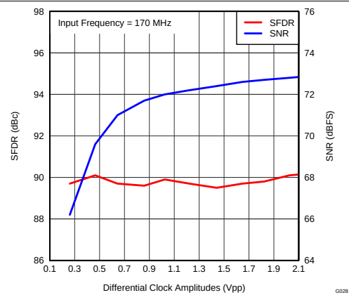
图 33. Performance vs Clock Amplitude (170 MHz)
