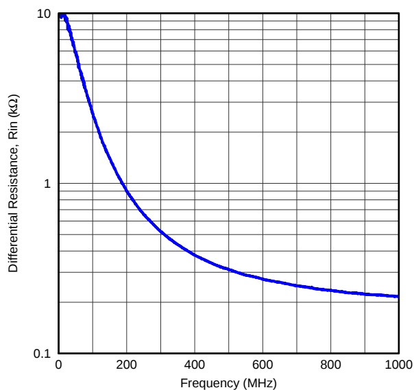
Figure 55. ADC Analog Input Resistance ( R_{IN} ) Across Frequency
