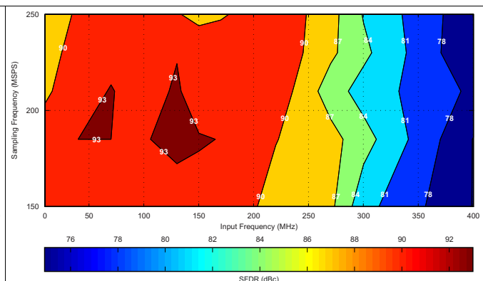
Figure 34. Spurious-Free Dynamic Range (6-dB Gain)
