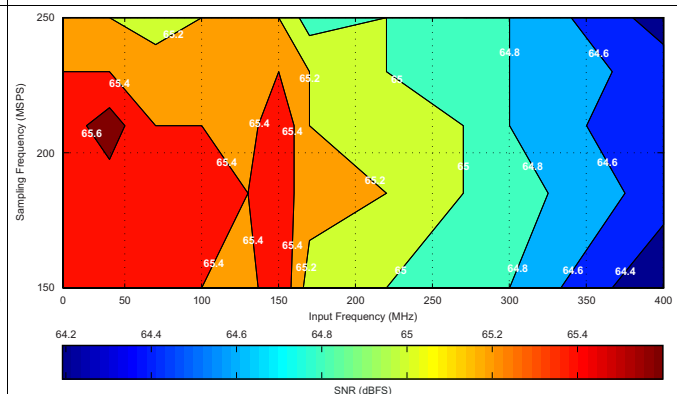
Figure 36. Signal-to-Noise Ratio (6-dB Gain)
