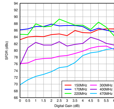
图 7-35. SFDR vs Gain and Input Frequency
