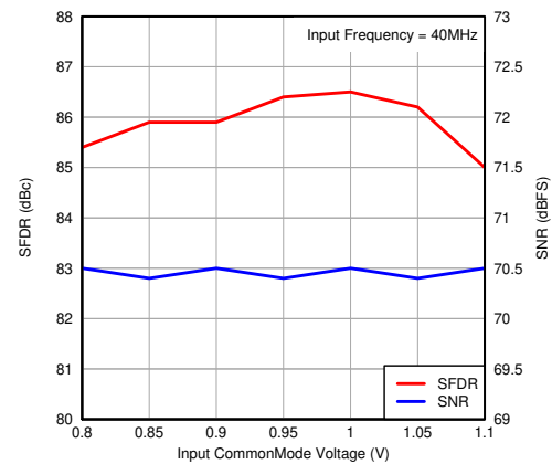
图 7-81. Performance vs Input Common-Mode Voltage
