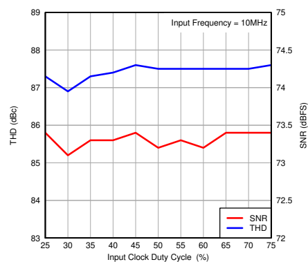
图 7-45. Performance vs Input Clock Duty Cycle
