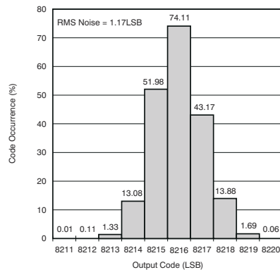
图 7-27. Output Noise Histogram (With Inputs Shorted to VCM)
