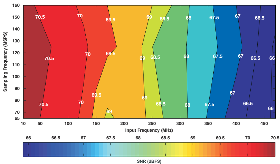
图 7-133. ADS422x Signal-to-Noise Ratio (0-dB Gain)
