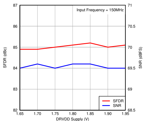
图 7-120. Performance vs DRVDD Supply Voltage
