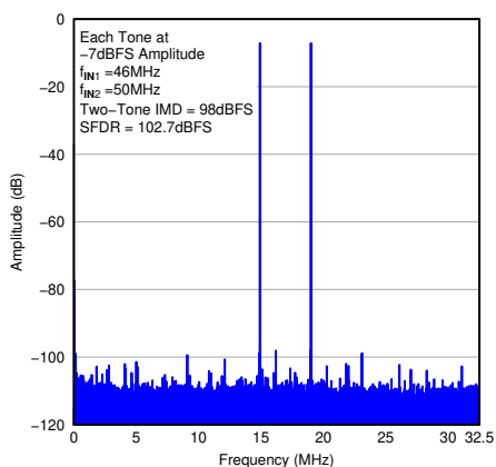
图 7-52. FFT for Two-Tone Input Signal
