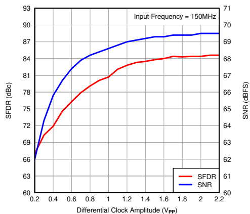
图 7-122. Performance vs Input Clock Amplitude
