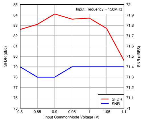
图 7-61. Performance vs Input Common-Mode Voltage
