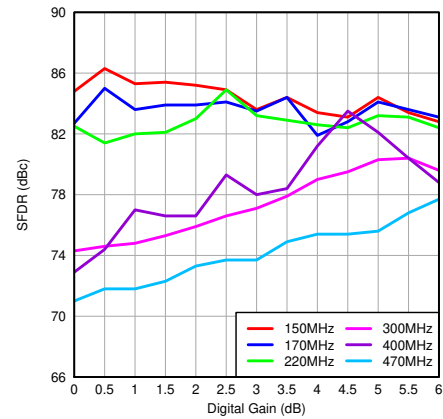
图 7-77. SFDR vs Gain and Input Frequency
