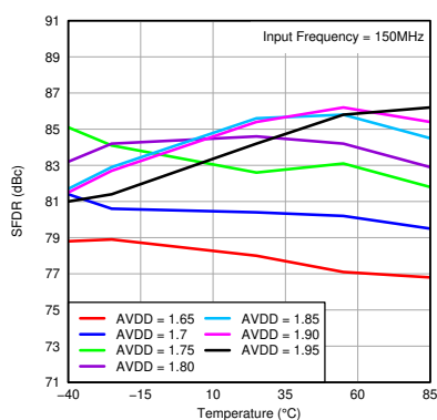
图 7-20. SFDR vs Temperature and AVDD Supply
