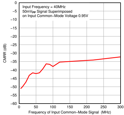
图 7-124. CMRR vs Test Signal Frequency
