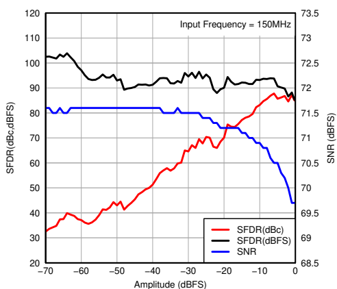
图 7-96. Performance vs Input Amplitude
