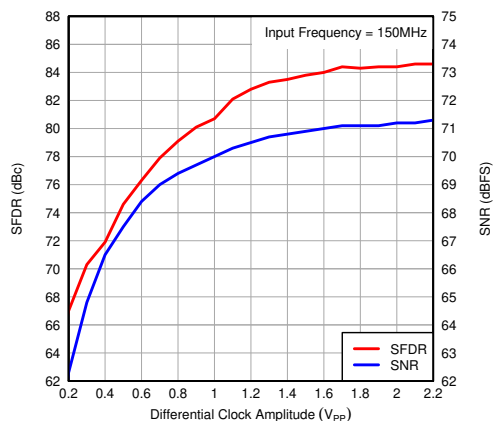
图 7-66. Performance vs Input Clock Amplitude
