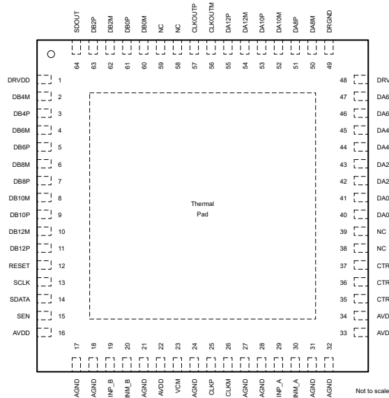
图 6-1. ADS4246, ADS4245, and ADS4242 RGC Package 64-Pin VQFN With Exposed Thermal Pad LVDS Mode (Top View)
