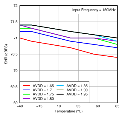
图 7-21. SNR vs Temperature and AVDD Supply
