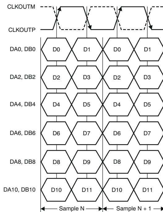
图 7-4. ADS4226/25/22 LVDS Interface Timing Diagram
