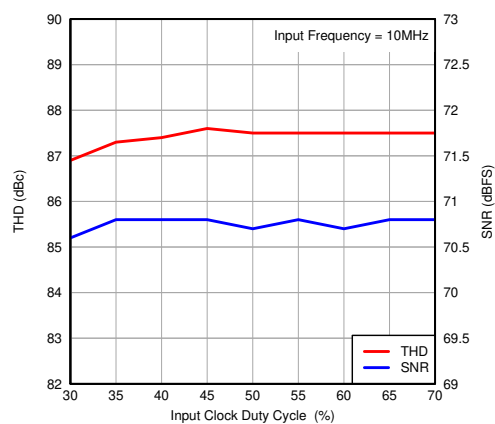
图 7-103. Performance vs Input Clock Duty Cycle
