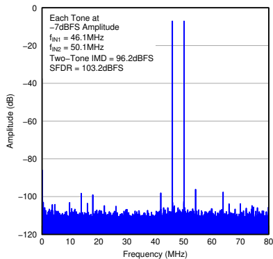
图 7-10. FFT for Two-Tone Input Signal
