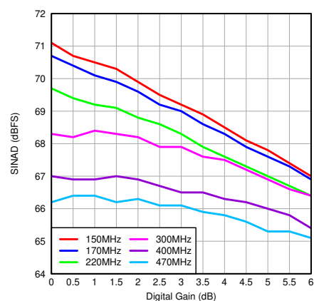
图 7-57. SINAD vs Gain and Input Frequency
