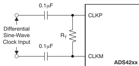
图 8-10. Differential Sine-Wave Clock Driving Circuit
