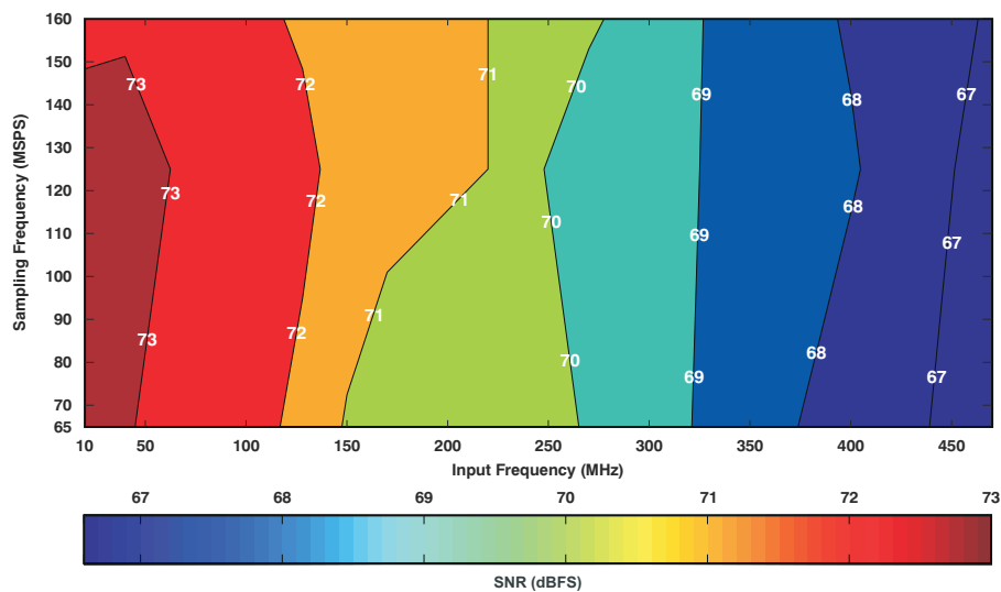
图 7-131. ADS424x Signal-to-Noise Ratio (0-dB Gain)
