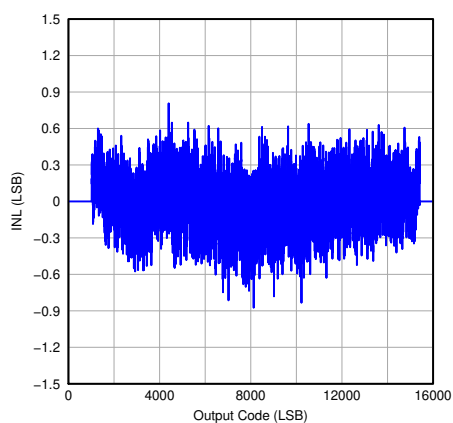
图 7-68. Integrated Nonlinearity
