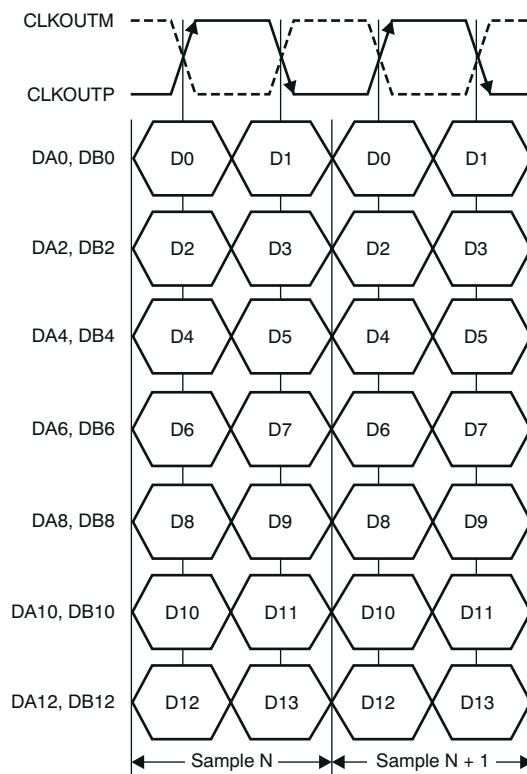
图 7-3. ADS4246/45/42 LVDS Interface Timing Diagram
