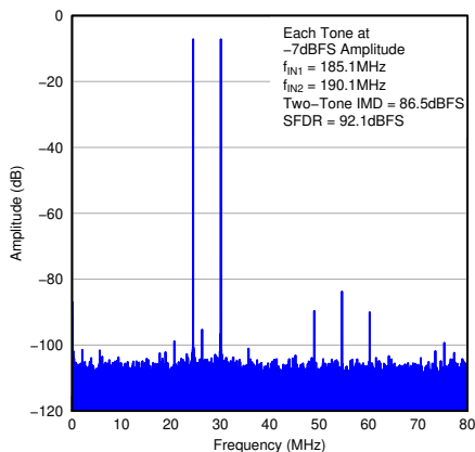
图 7-72. FFT for Two-Tone Input Signal
