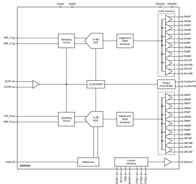
ADS4222/25/26/42/45/46 方框图
