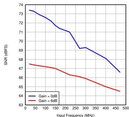
图 7-33. SNR vs Input Frequency
