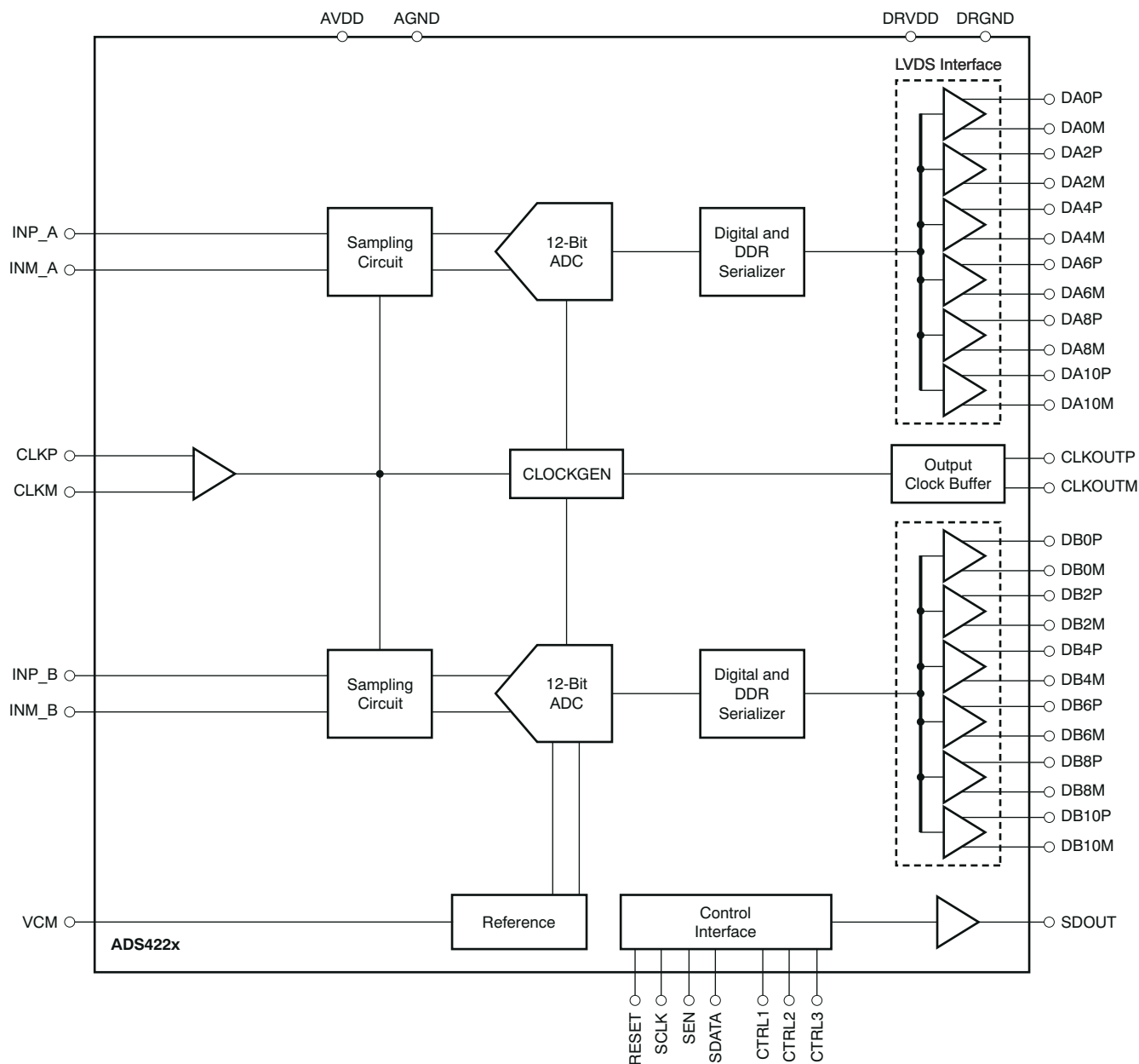
图 8-2. ADS4226, 25, 22 Block Diagram
