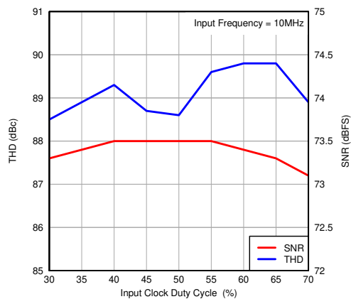
图 7-67. Performance Across Input Clock Duty Cycle
