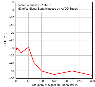
图 7-125. PSRR vs Test Signal Frequency
