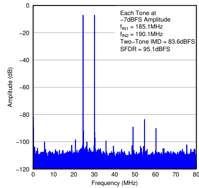
图 7-9. FFT for Two-tone Input Signal
