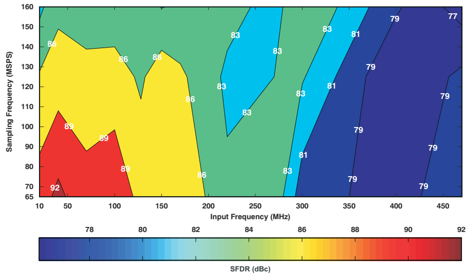
图 7-130. Spurious-Free Dynamic Range (6-dB Gain)
