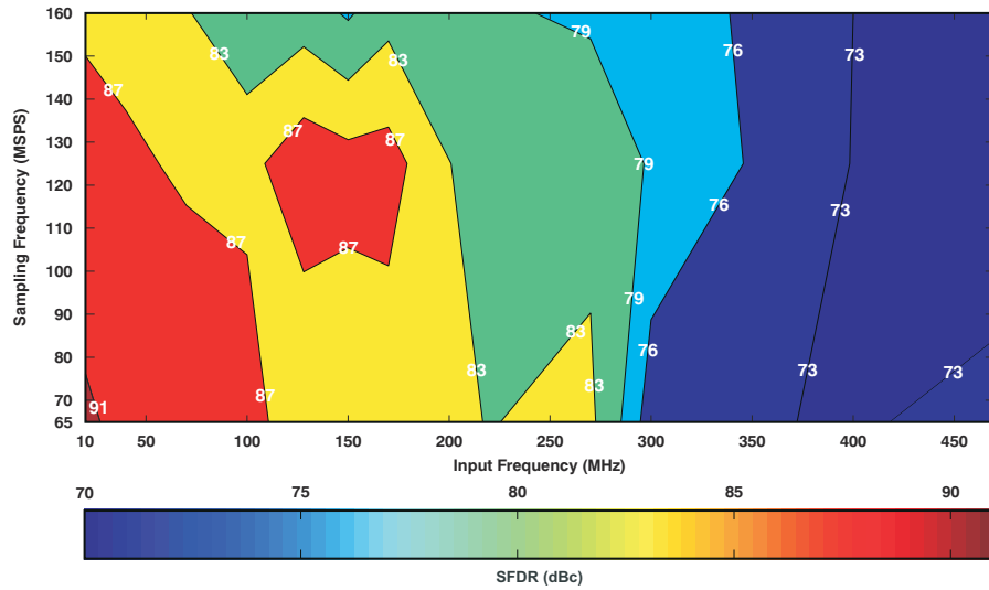
图 7-129. Spurious-Free Dynamic Range (0-dB Gain)
