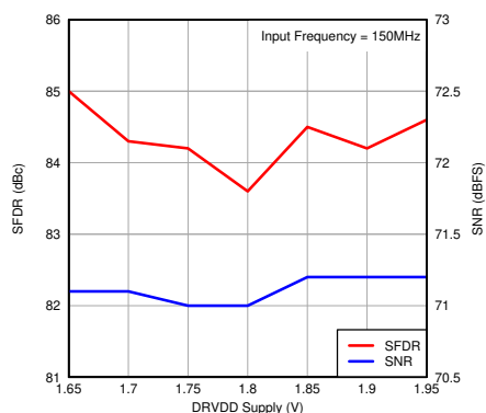
图 7-22. Performance vs DRVDD Supply Voltage
