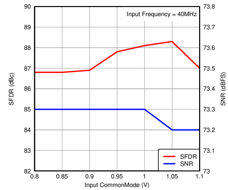
图 7-39. Performance vs Input Common-Mode Voltage
