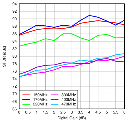
图 7-112. SFDR vs Gain and Input Frequency
