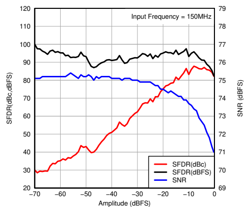
图 7-59. Performance vs Input Amplitude
