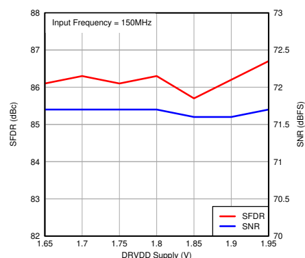
图 7-43. Performance vs DRVDD Supply Voltage
