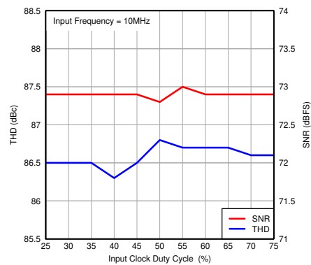
图 7-25. Performance vs Input Clock Duty Cycle
