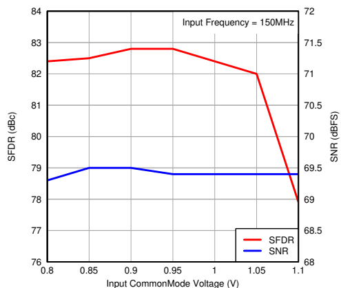
图 7-82. Performance vs Input Common-Mode Voltage
