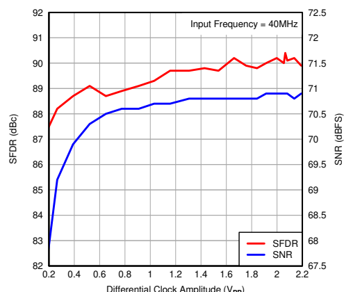
图 7-121. Performance vs Input Clock Amplitude
