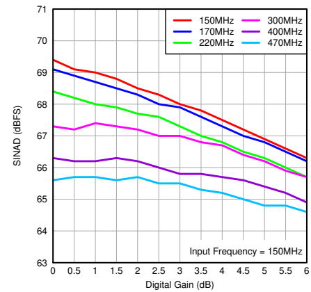
图 7-113. SINAD vs Gain and Input Frequency
