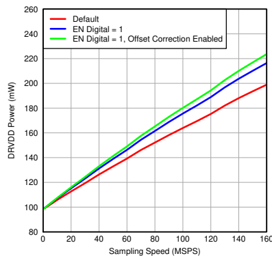
图 7-128. Digital Power in Various Modes (LVDS)
