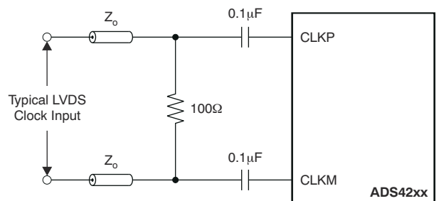
图 8-11. LVDS Clock Driving Circuit
