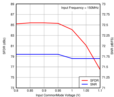
图 7-40. Performance vs Input Common-Mode Voltage
