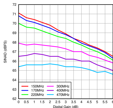
图 7-15. SINAD vs Gain and Input Frequency
