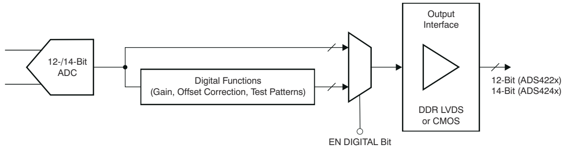
图 8-15. Digital Processing Block
