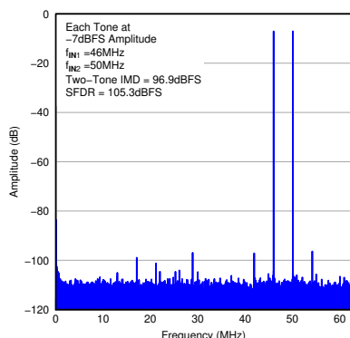
图 7-32. FFT for Two-Tone Input Signal
