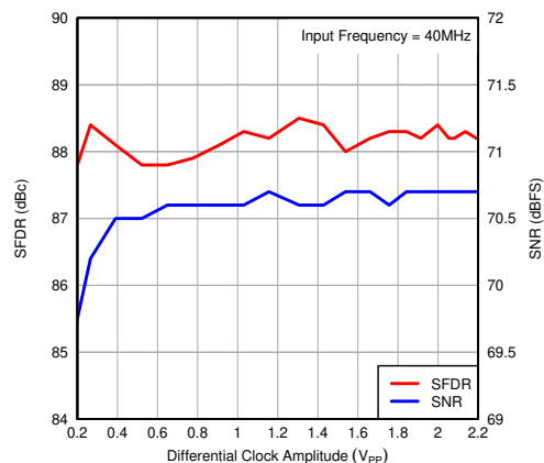
图 7-101. Performance vs Input Clock Amplitude
