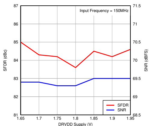
图 7-84. Performance vs DRVDD Supply Voltage
