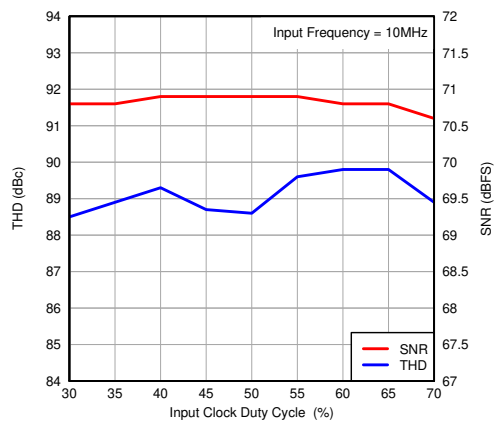
图 7-123. Performance vs Input Clock Duty Cycle
