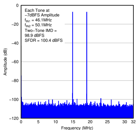
图 7-108. FFT for Two-Tone Input Signal
