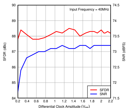
图 7-44. Performance vs Input Clock Amplitude
