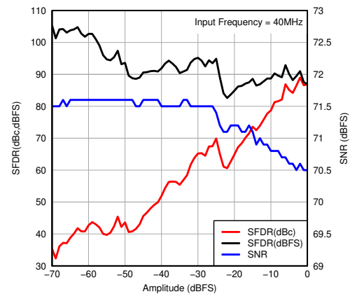
图 7-79. Performance vs Input Amplitude
