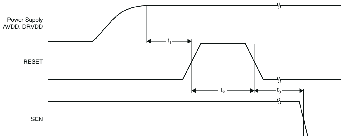
图 8-18. Serial Readout Timing Diagram
