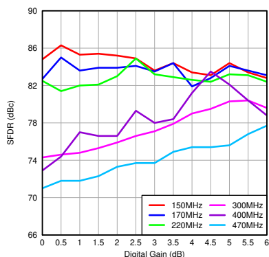
图 7-14. SFDR vs Gain and Input Frequency
