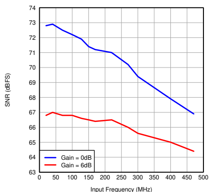
图 7-12. SNR vs Input Frequency
