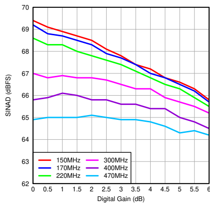
图 7-78. SINAD vs Gain and Input Frequency
