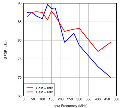
图 7-91. SFDR vs Input Frequency
