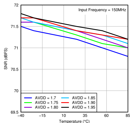
图 7-63. SNR vs Temperature and AVDD Supply
