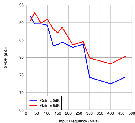
图 7-109. SFDR vs Input Frequency
