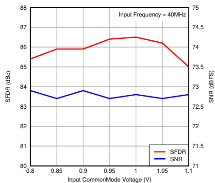
图 7-18. Performance vs Input Common-Mode Voltage
