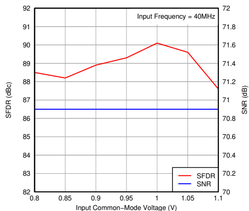
图 7-116. Performance vs Input Common-Mode Voltage
