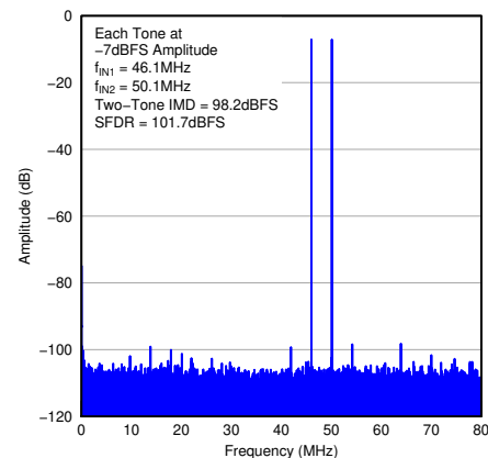
图 7-73. FFT for Two-Tone Input Signal
