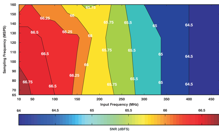
图 7-134. ADS422x Signal-to-Noise Ratio (6-dB Gain)
