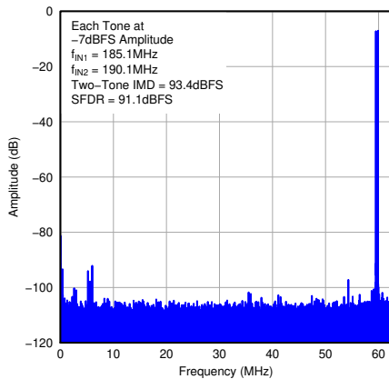
图 7-90. FFT for Two-Tone Input Signal
