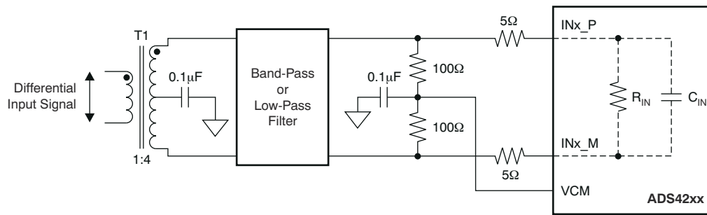
图 8-9. Drive Circuit with a 1:4 Transformer
