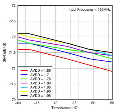
图 7-42. SNR vs Temperature and AVDD Supply
