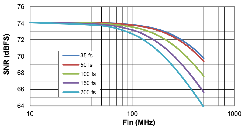
图 9-2. SNR versus Input Frequency and External Clock Jitter
