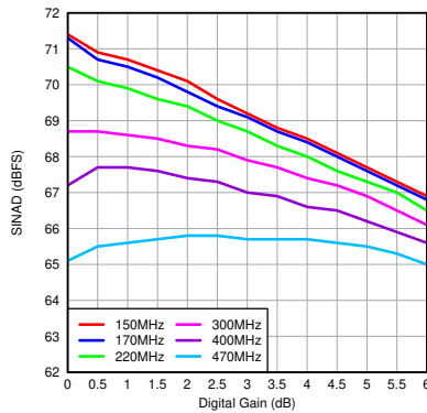
图 7-36. SINAD vs Gain and Input Frequency
