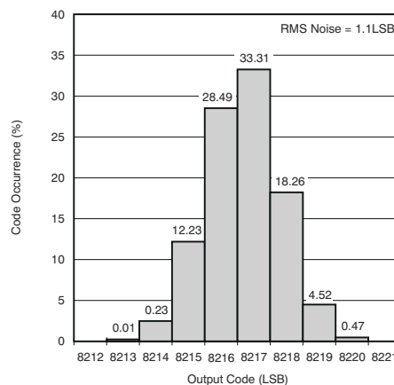
图 7-69. Output Noise Histogram (With Inputs Shorted to VCM)
