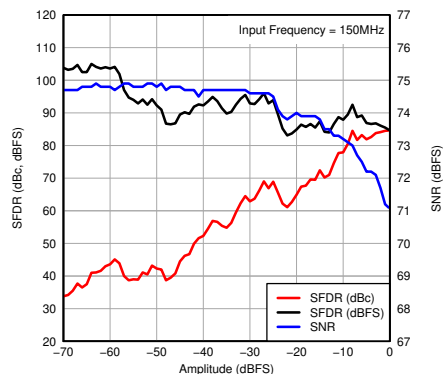
图 7-17. Performance vs Input Amplitude
