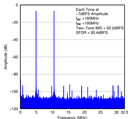
图 7-51. FFT for Two-Tone Input Signal
