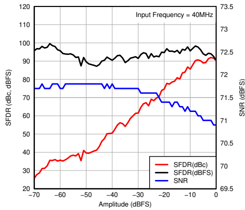
图 7-114. Performance vs Input Amplitude
