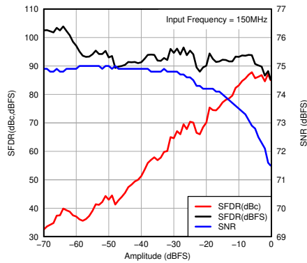
图 7-38. Performance vs Input Amplitude
