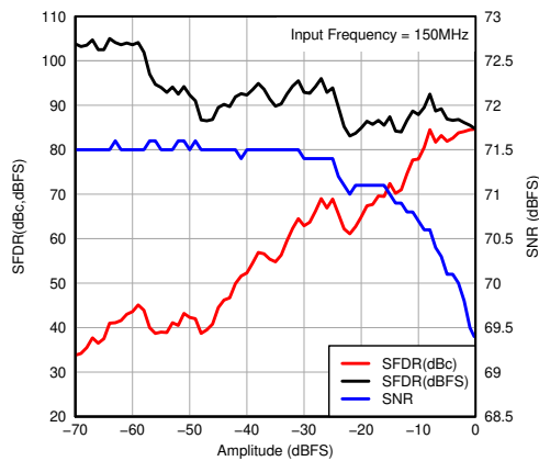
图 7-80. Performance vs Input Amplitude
