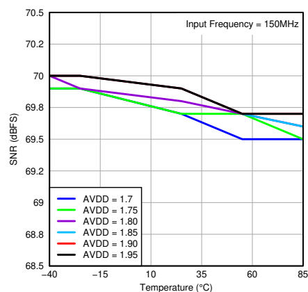
图 7-99. SNR vs Temperature and AVDD Supply
