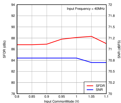
图 7-97. Performance vs Input Common-Mode Voltage
