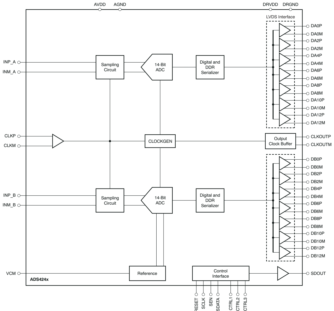
图 8-1. ADS4246, 45, 42 Block Diagram
