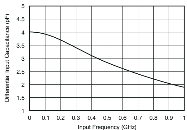
图 8-5. ADC Analog Input Capacitance ( C_{IN} ) Across Frequency
