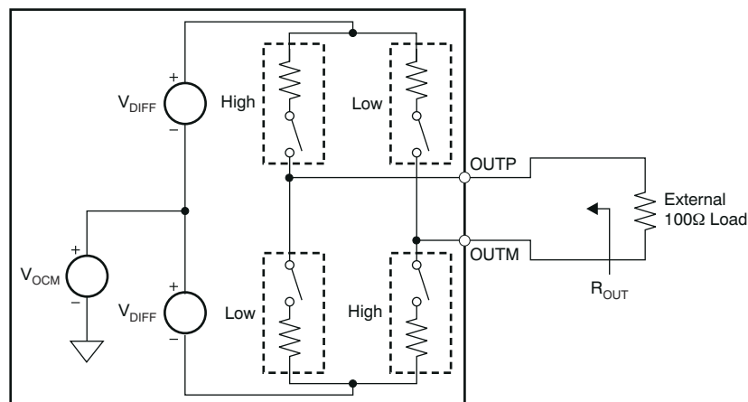
图 8-22. LVDS Buffer Equivalent Circuit
