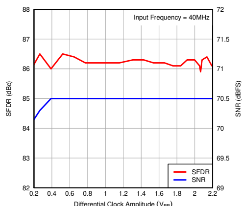
图 7-85. Performance vs Input Clock Amplitude
