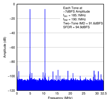
图 7-107. FFT for Two-Tone Input Signal
