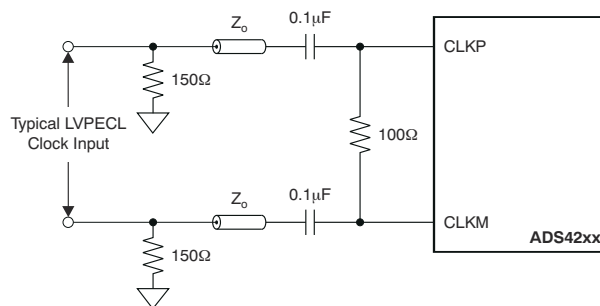
图 8-12. LVPECL Clock Driving Circuit
