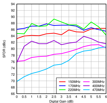
图 7-94. SFDR vs Gain and Input Frequency
