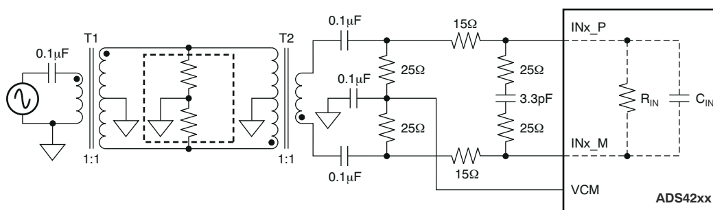
图 8-6. Drive Circuit with Low Bandwidth (for Low Input Frequencies Less Than 150 MHz)
