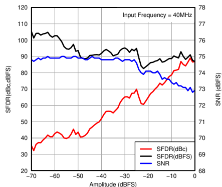
图 7-16. Performance vs Input Amplitude
