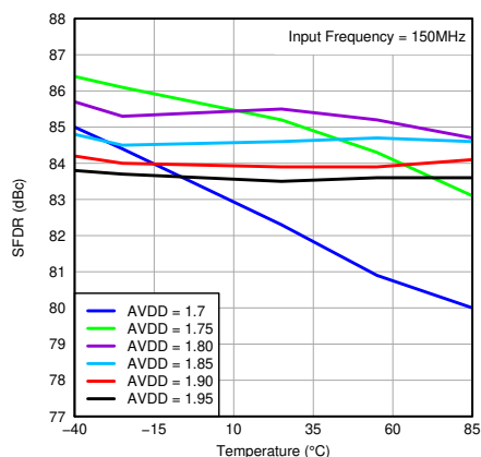
图 7-118. SFDR vs Temperature and AVDD Supply
