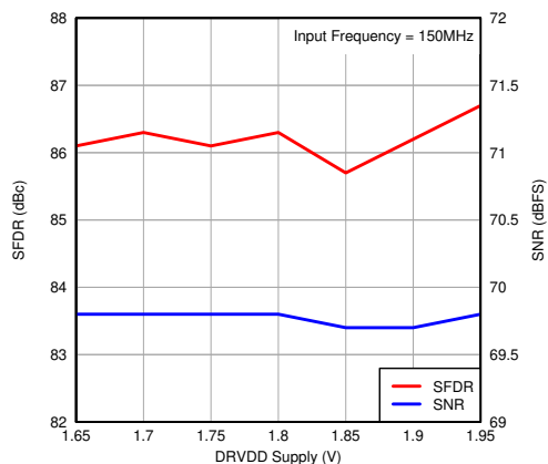
图 7-100. Performance vs DRVDD Supply Voltage
