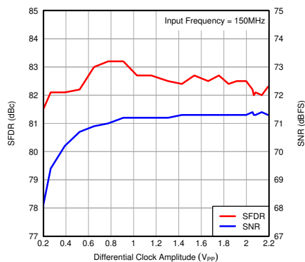
图 7-24. Performance vs Input Clock Amplitude
