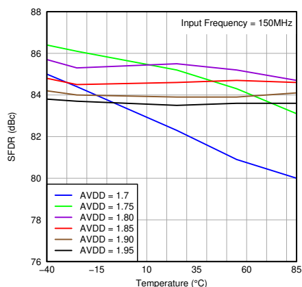
图 7-62. SFDR vs Temperature and AVDD Supply
