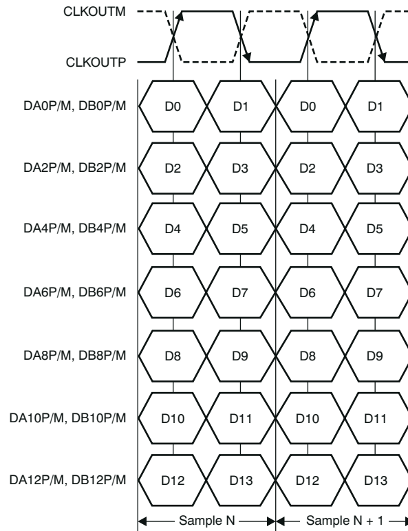
图 8-21. DDR LVDS Interface Timing
