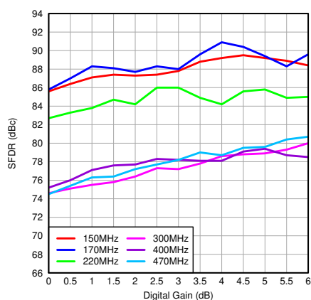
图 7-56. SFDR vs Gain and Input Frequency
