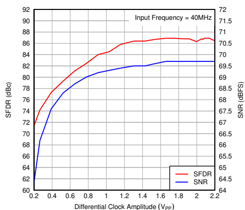
图 7-102. Performance vs Input Clock Amplitude
