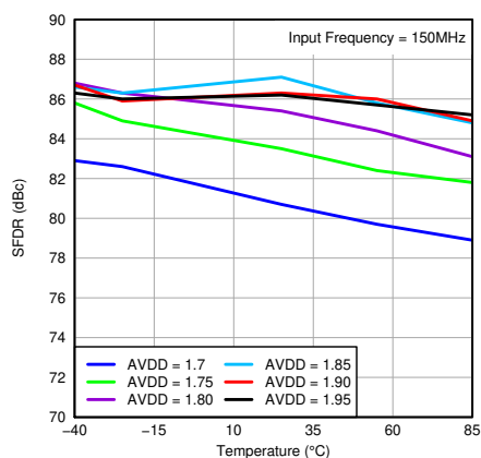
图 7-98. SFDR vs Temperature and AVDD Supply
