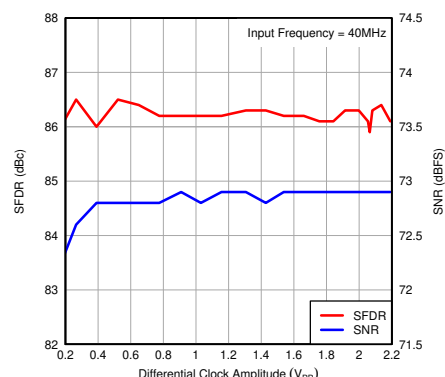
图 7-23. Performance vs Input Clock Amplitude
