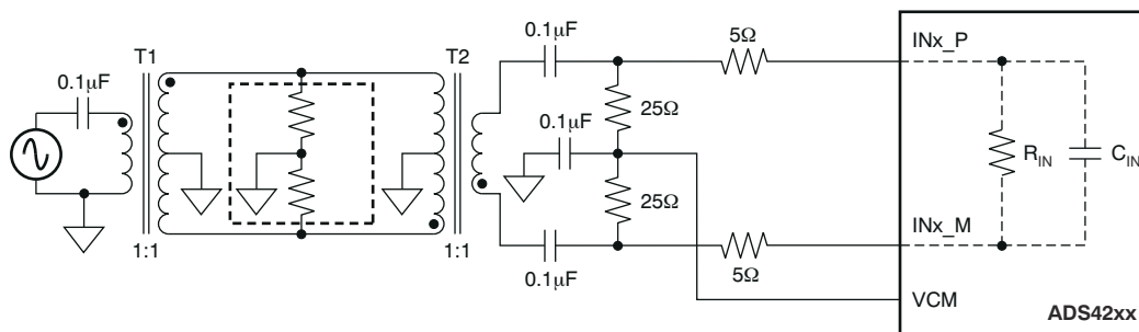
图 8-8. Drive Circuit with Very High Bandwidth (Greater than 270 MHz)
