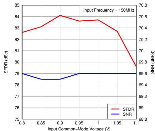
图 7-117. Performance vs Input Common-Mode Voltage
