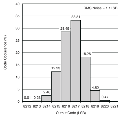
图 7-47. Output Noise Histogram (With Inputs Shorted to VCM)
