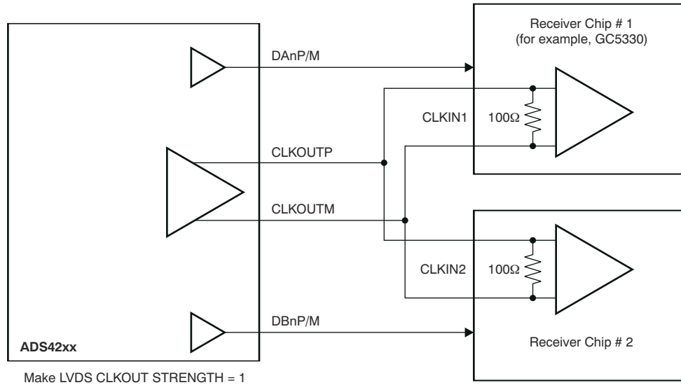
图 8-23. LVDS Buffer Differential Termination
