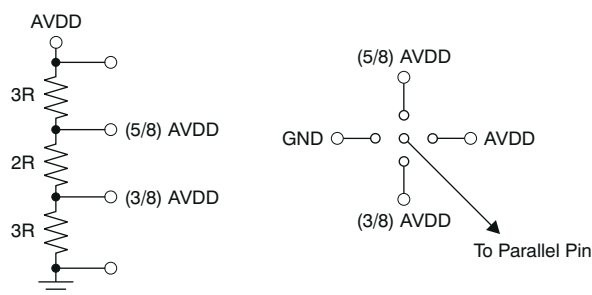
图 8-16. Simple Scheme to Configure the Parallel Pins
