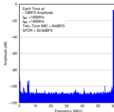
图 7-31. FFT for Two-Tone Input Signal
