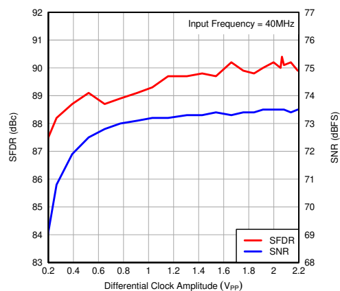
图 7-65. Performance vs Input Clock Amplitude
