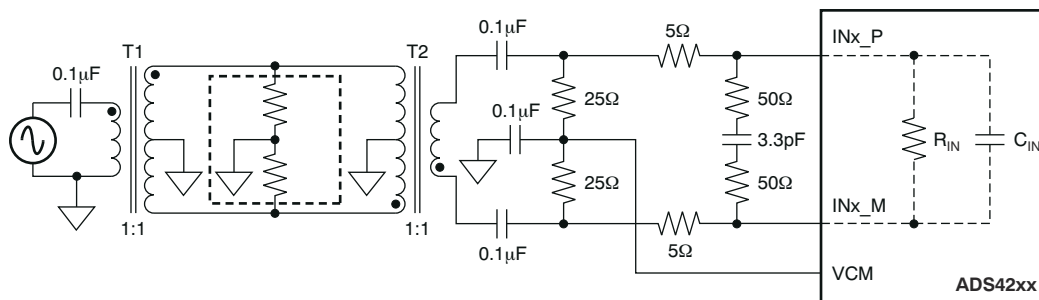
图 8-7. Drive Circuit with High Bandwidth (for High Input Frequencies Greater Than 150 MHz and Less Than 270 MHz)
