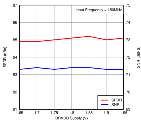
图 7-64. Performance vs DRVDD Supply Voltage
