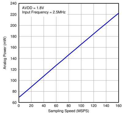
图 7-126. Analog Power vs Sampling Frequency
