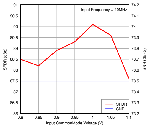
图 7-60. Performance vs Input Common-Mode Voltage
