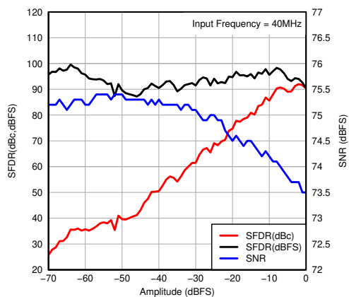
图 7-58. Performance vs Input Amplitude
