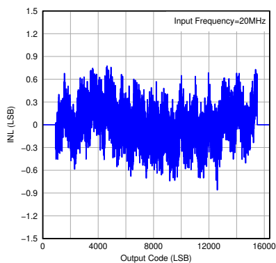
图 7-26. Integrated Nonlinearity
