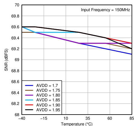
图 7-83. SNR vs Temperature and AVDD Supply
