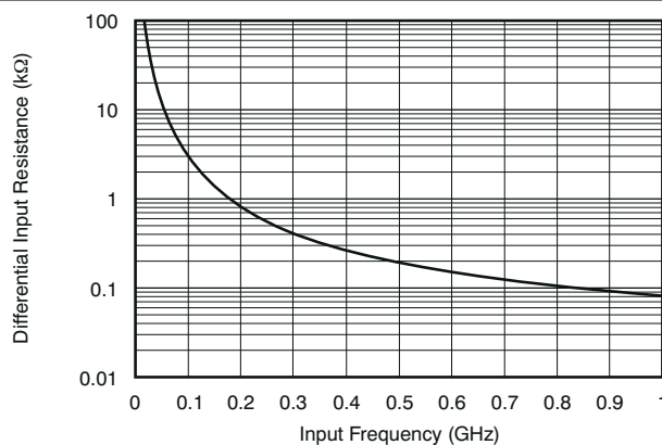
图 8-4. ADC Analog Input Resistance ( R_{IN} ) Across Frequency
