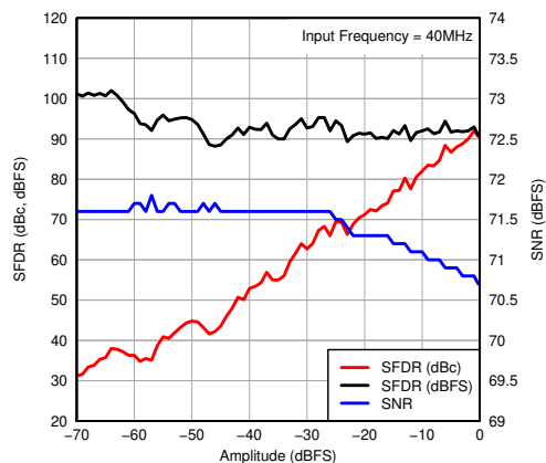
图 7-95. Performance vs Input Amplitude
