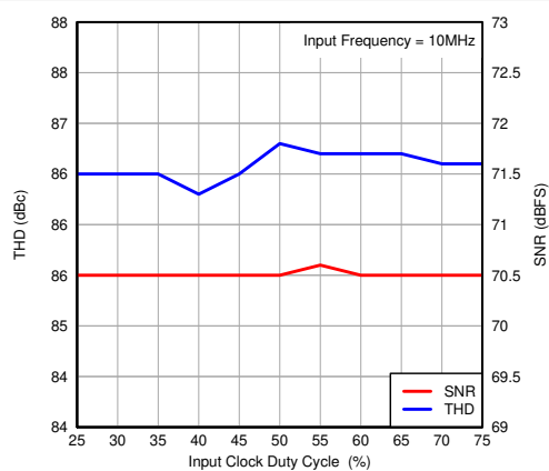
图 7-87. Performance vs Input Clock Duty Cycle
