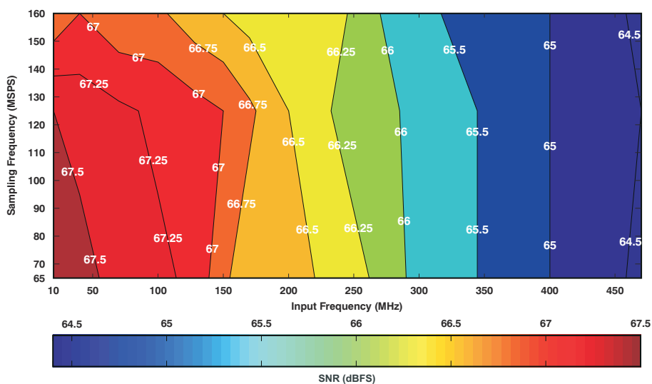
图 7-132. ADS424x Signal-to-Noise Ratio (6-dB Gain)
