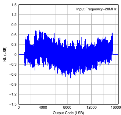
图 7-46. Integrated Nonlinearity
