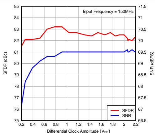
图 7-86. Performance vs Input Clock Amplitude
