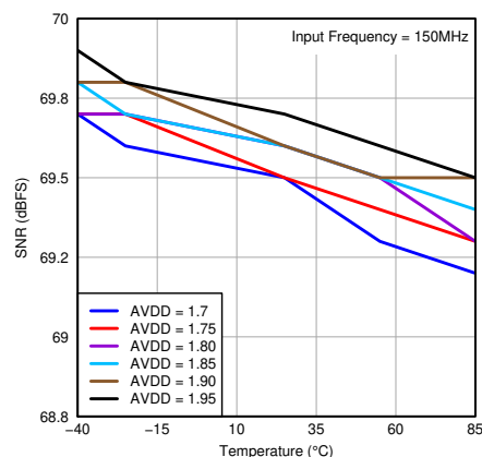
图 7-119. SNR vs Temperature and AVDD Supply
